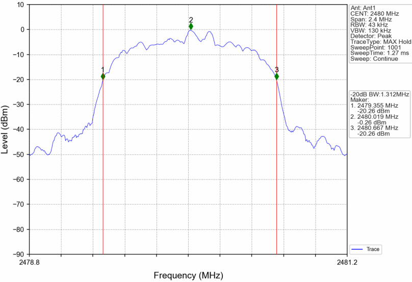
8DPSK_3DH5_HCH_2480MHz_Ant1_NTNV
