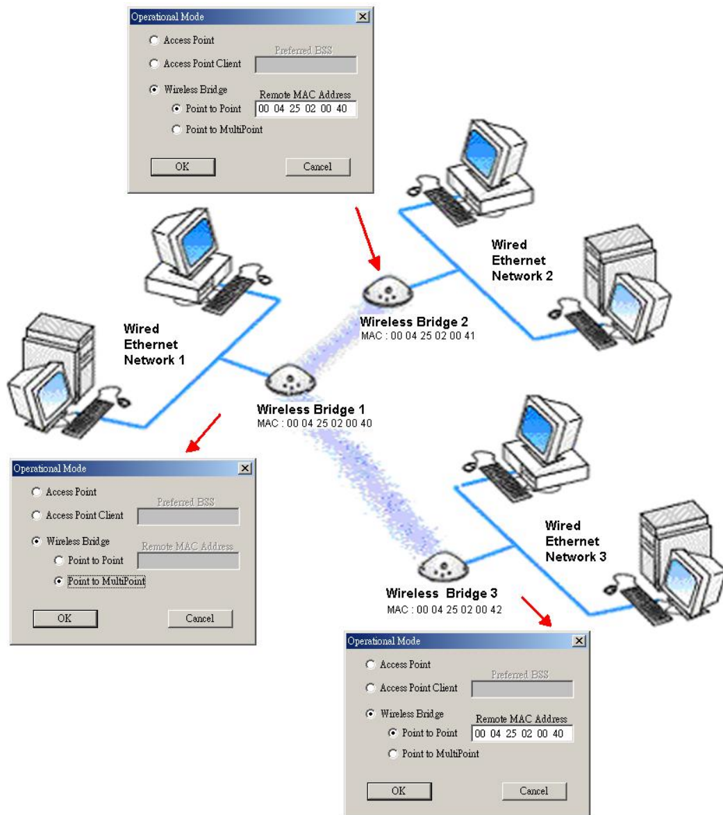
Figure 3-4 Wireless Bridge – Point to Multipoint
