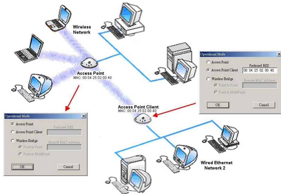
Figure 3-2 Access Point Client
