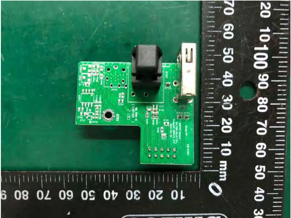
Internal Photos M/N: Soundbar
