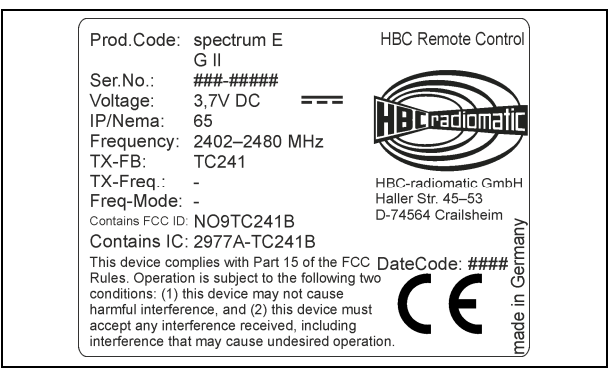
Figure 1: Example type plate of a host device
