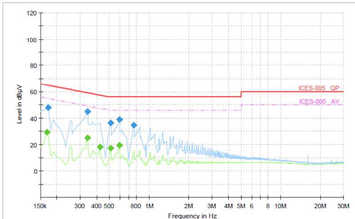
Figure 1: Spectral Diagrams, Conducted Emission, 150kHz - 30MHz, L
