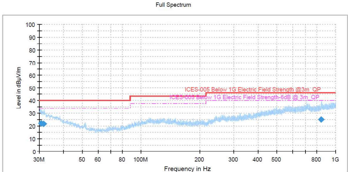
Figure 3: Spectral Diagrams, Radiated Emission, 30MHz-1000MHz, Horizontal polarization
