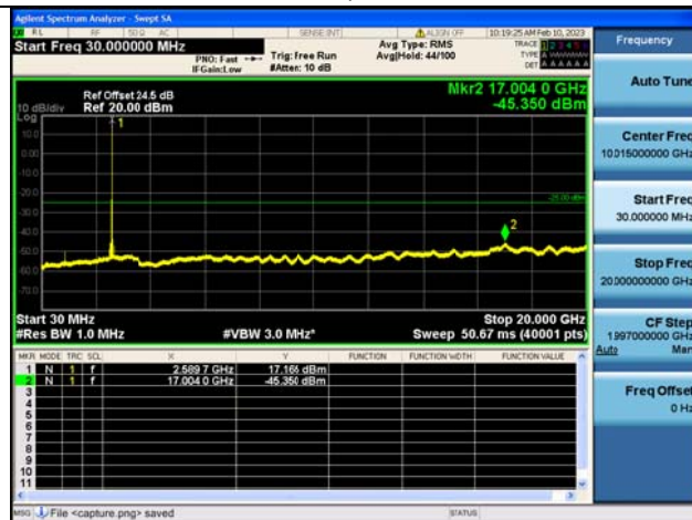
Band41C-30M-20G / 15MHz+20MHz /1RB+1RB/ QPSK / Mid CH
