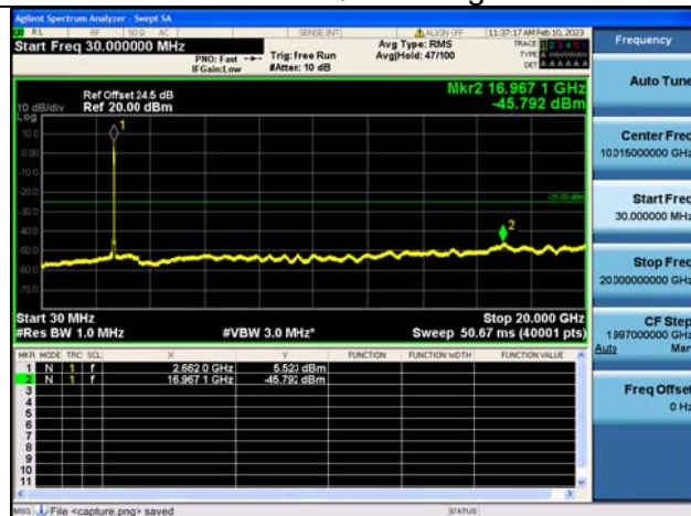
Band41C-30M-20G / 20MHz+10MHz /100RB+50RB/ QPSK / High CH
