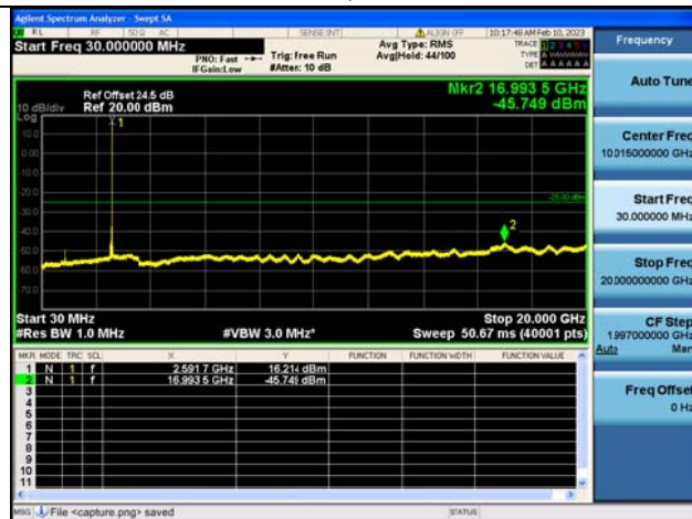
Band41C-30M-20G / 15MHz+15MHz /1RB+1RB/ QPSK / Mid CH
