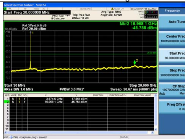
Band41C-30M-20G / 10MHz+15MHz /1RB+1RB/ QPSK / High CH
