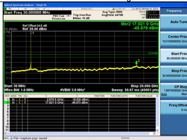
Band41C-30M-20G / 20MHz+10MHz /1RB+1RB/ QPSK / High CH
