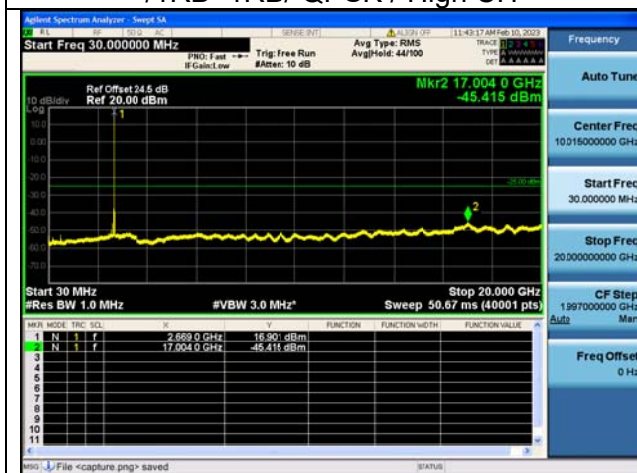
Band41C-30M-20G / 20MHz+20MHz /1RB+1RB/ QPSK / High CH
