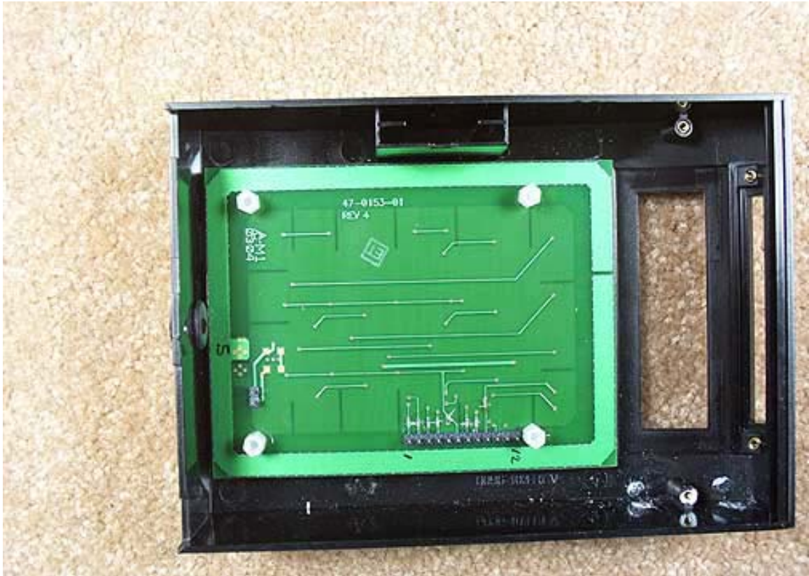
Keypad PCB Back
