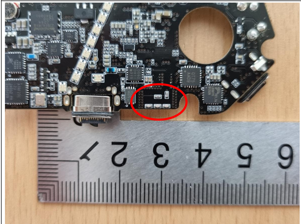
BT2 Antenna
