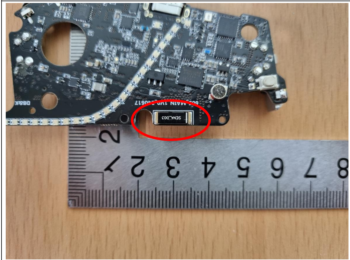
BT1 Antenna
