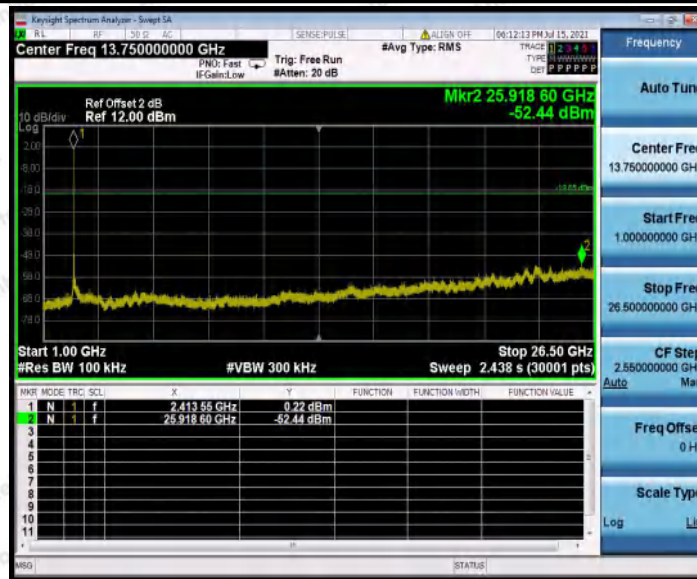
11B_Ant2_2412_0~Reference
