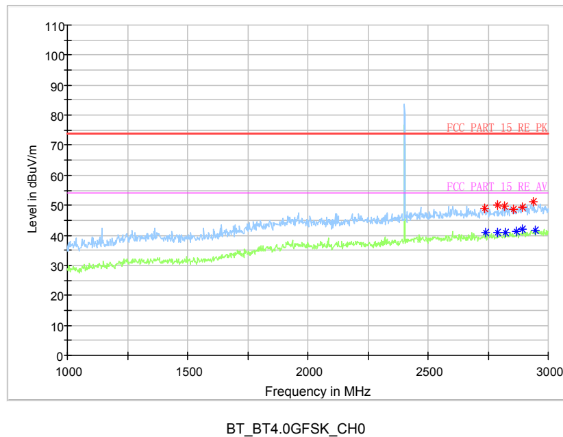
Fig.22 Radiated Spurious Emission (GFSK, Ch0, 1 GHz ~3 GHz)
