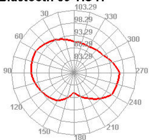
Bluetooth 39 TIS H
