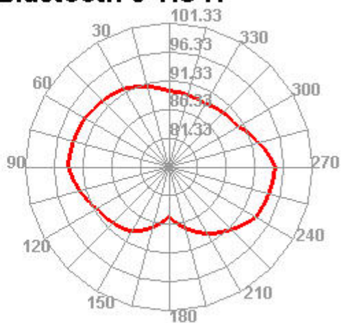
Bluetooth 0 TIS H
