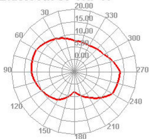
Bluetooth 39 TRP H
