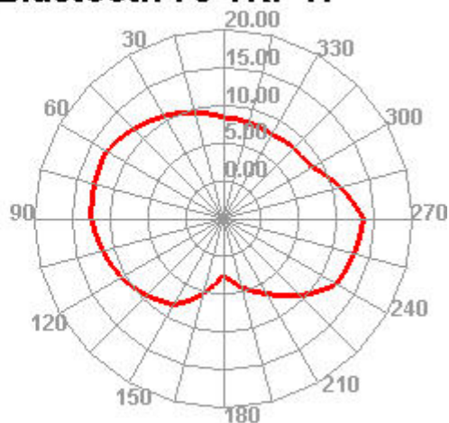
Bluetooth 78 TRP H
