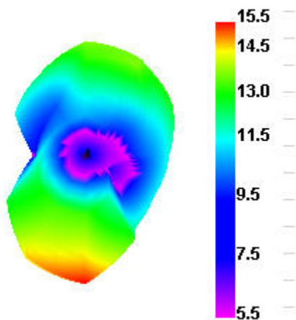
Bluetooth 39 TRP
