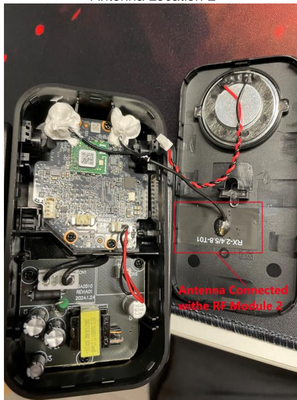
Antenna Location-2
