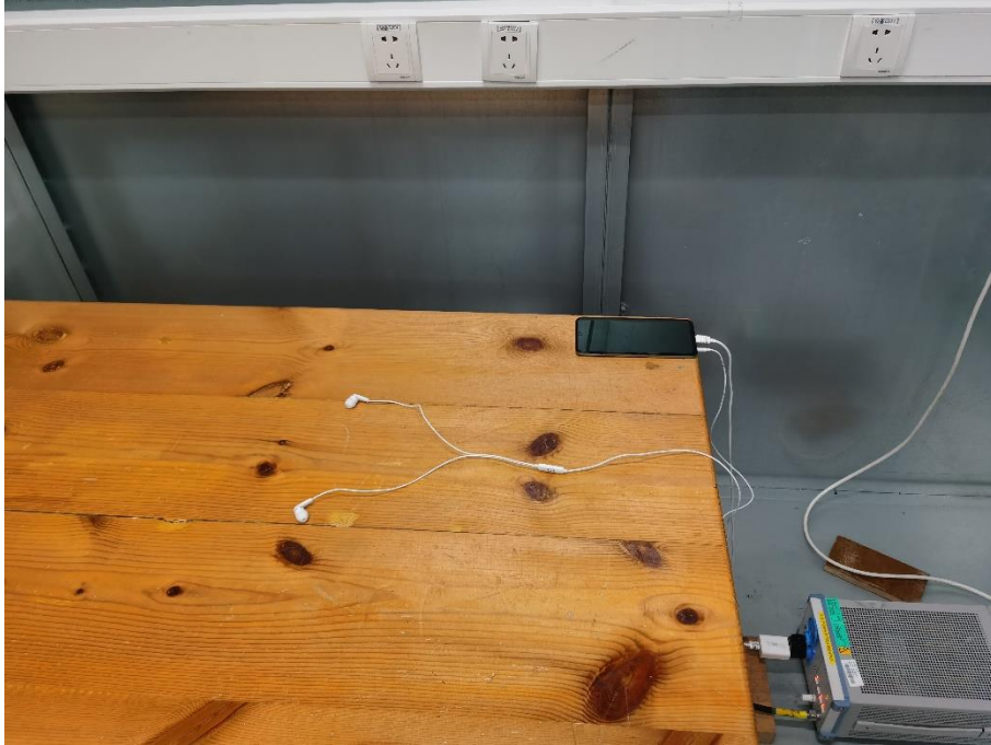
17. Conducted Emission (Part 15C, Bluetooth/Wi-Fi)
