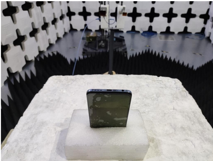
14. Radiated Emissions (Par22/24/27, 18GHz -26.5GHz)
