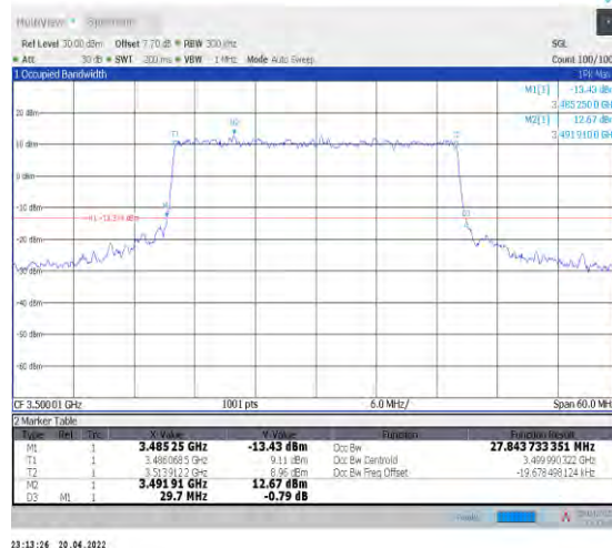
1-N78-3450-3550--30-30-M-8-CP-64QAM-Outer_Ful I-78@0-Ant1-27.844-29.700-≤30-PASS
