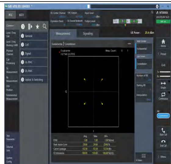
1-N78-3450-3550--30-100-M-2-DFT-QPSK-Outter_Full-270@0-Ant1-see graph-PASS
