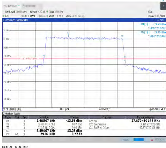
1-N78-3450-3550--30-30-M-7-CP-16QAM-Outer_Full -78@0-Ant1-27.87-29.820-≤30-PASS
