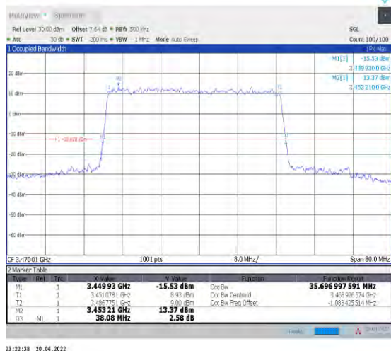
1-N78-3450-3550--30-40-L-5-DFT-256QAM-Outer_Full-100@0-Ant1-35.697-38.080-≤40-PASS
