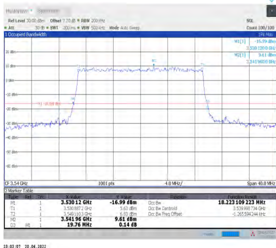
1-N78-3450-3550--30-20-H-9-CP-256QAM-Outer_Fu II-51@0-Ant1-18.223-19.760-≤20-PASS
