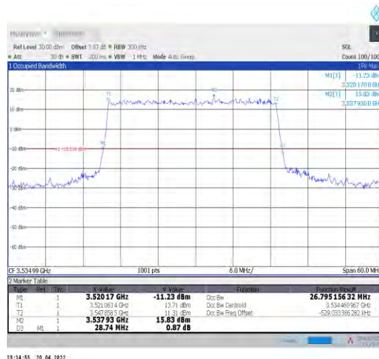
1-N78-3450-3550--30-30-H-1-DFT-QPSK-Outer_Full -75@0-Ant1-26.795-28.740-≤30-PASS
