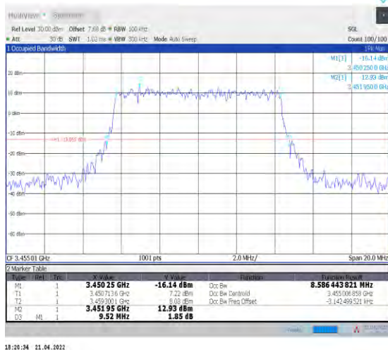
1-N78-3450-3550--30-10-L-3-DFT-16QAM-Outter_Full-24@0-Ant1-8.586-9.520-≤10-PASS
