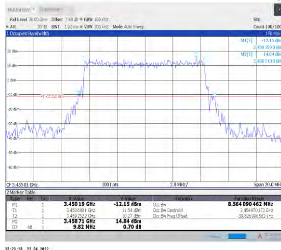
1-N78-3450-3550--30-10-L-2-DFT-PI2BPSK-Outter_Full-24@0-Ant1-8.564-9.820-≤10-PASS
