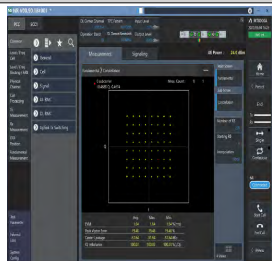
1-N78-3450-3550--30-100-M-4-DFT-64QAM-Outter_Full-270@0-Ant1-see graph-PASS
