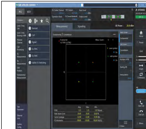
1-N78-3450-3550--30-100-M-1-DFT-PI2BPSK-Outter_Full-270@0-Ant1-see graph-PASS
