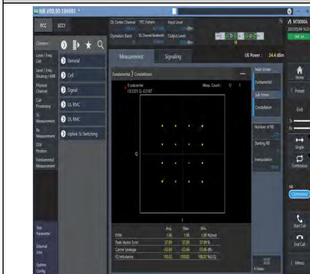
1-N78-3450-3550--30-100-M-3-DFT-16QAM-Outter_Full-270@0-Ant1-see graph-PASS
