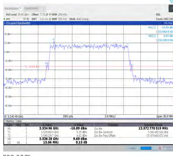
1-N78-3450-3550--30-15-H-9-CP-256QAM-Outer_Full -38@0-Ant1-13.573-15.060-≤15-PASS
