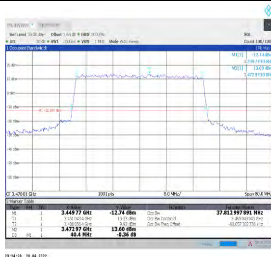
1-N78-3450-3550--30-40-L-8-CP-64QAM-Outer_Full-106@0-Ant1-37.813-40.400-≤40-PASS
