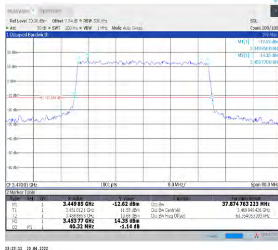
1-N78-3450-3550--30-40-L-6-CP-QPSK-Outer_Full-106@0-Ant1-37.875-40.320-≤40-PASS
