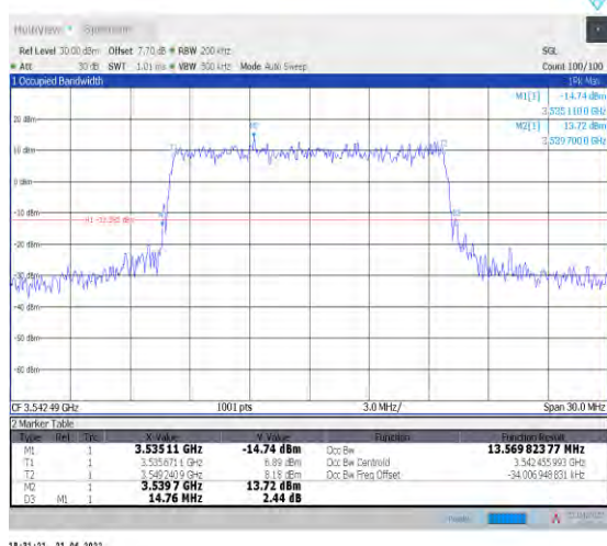
1-N78-3450-3550--30-15-H-8-CP-64QAM-Outer_Full -38@0-Ant1-13.57-14.760-≤15-PASS
