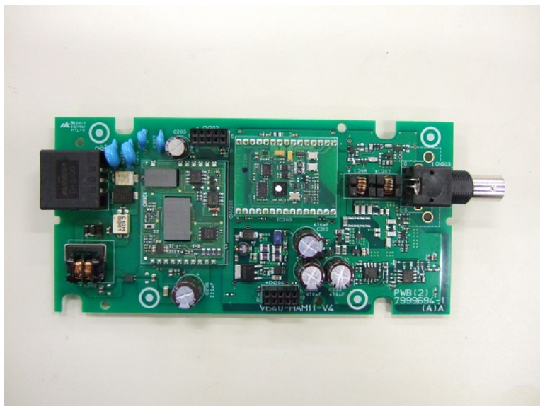
PCB(2) Side A without a shield plate
