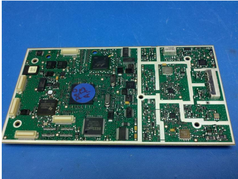
Satellite board – Topside view
