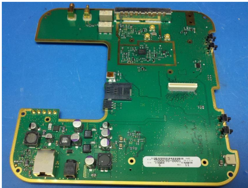
Interface board – Underside view
