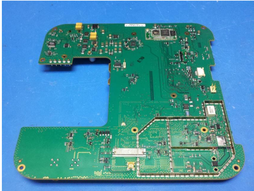
Interface board – Topside view, shield removed
