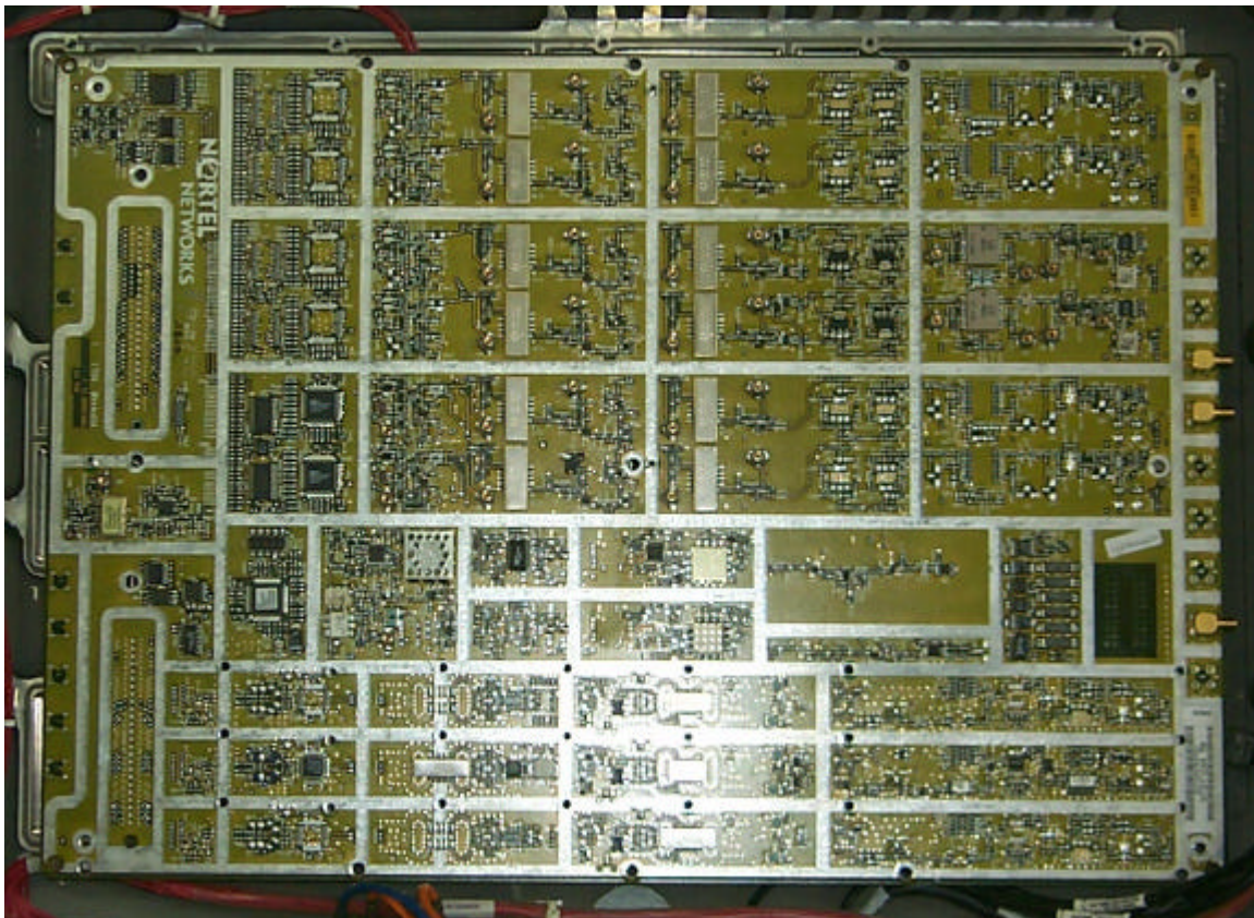
Nortel Networks 1900 MTRM RF Board NTGY12AA Top View
