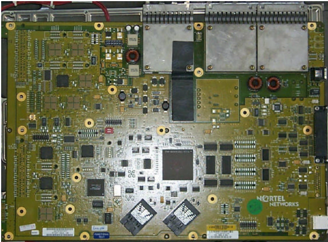
Nortel Networks 1900 MTRM Digital Board NTGY13AA Top View
