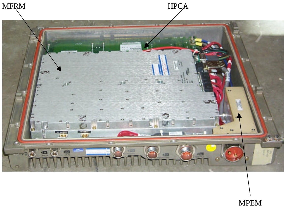
Nortel Networks 1900 MPAM Front/Top View
