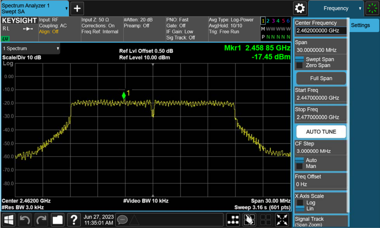
Figure 21: Power Spectral Density, 802.11n(HT20), 2462MHz
