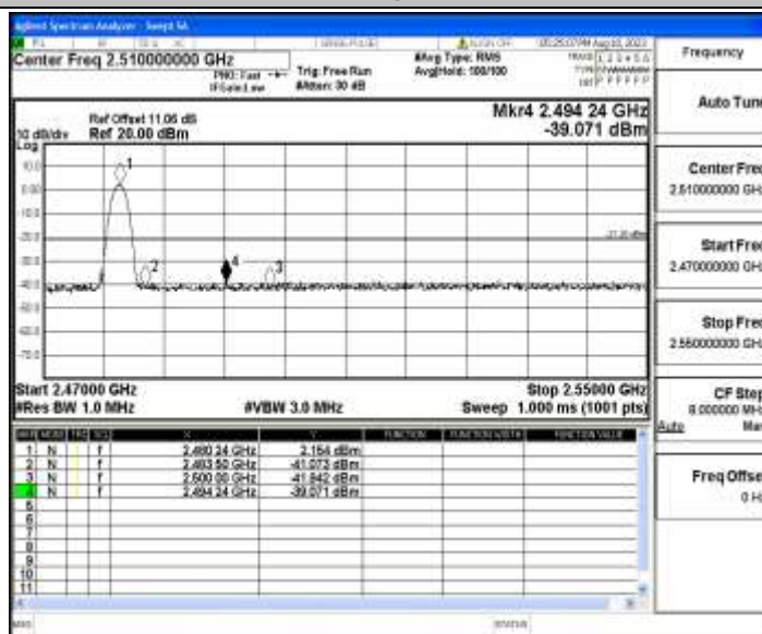
2DH5_Ant1_High_2480_Peak
