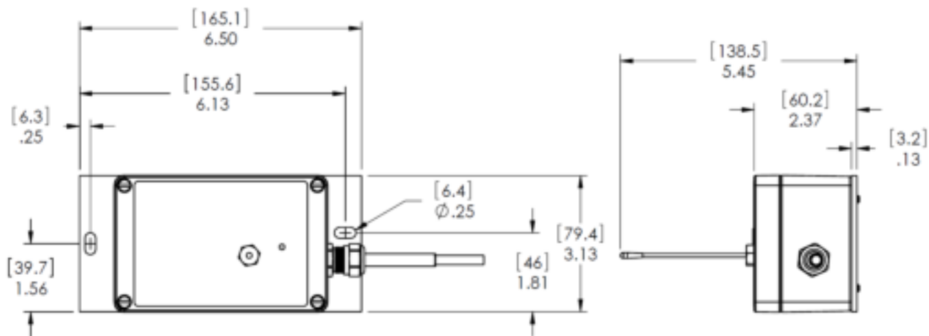
Slew sensor transmitter (not to scale)
