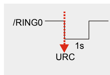
Figure 26: URC transmission
