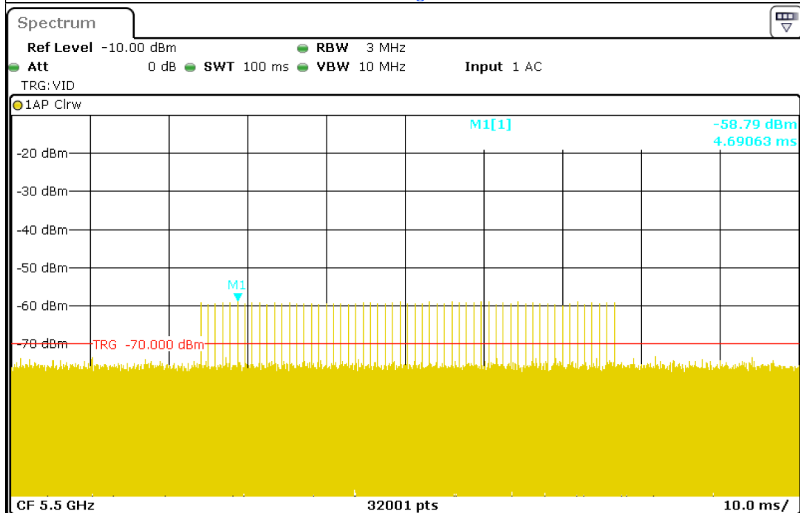
Radar Signal 1 (Test A)
