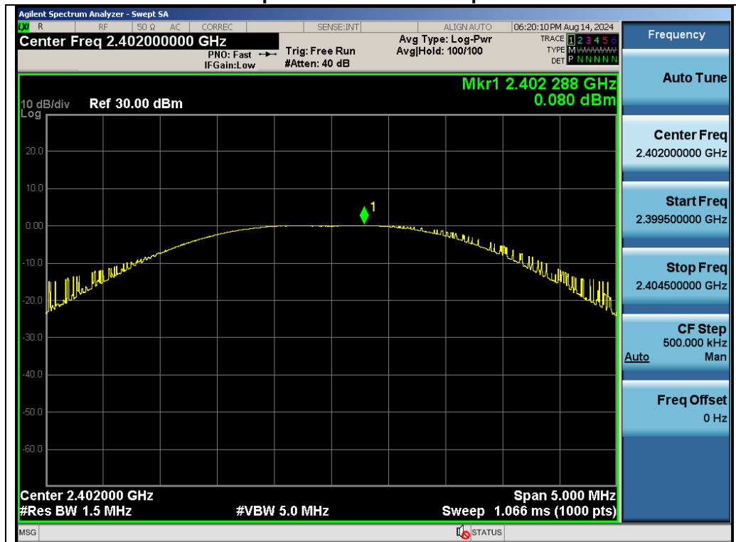
Test_Graph_2.4G_ANT1_2402_Peak Power
