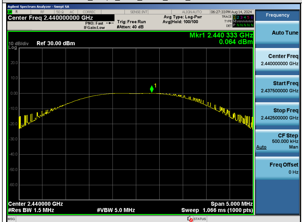
Test_Graph_2.4G_ANT1_2440_Peak Power
