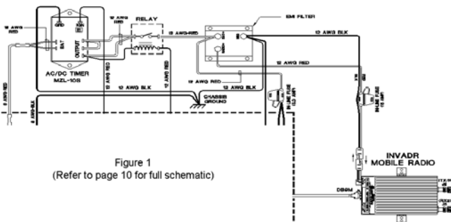
TRUNK COMPARTMENT
