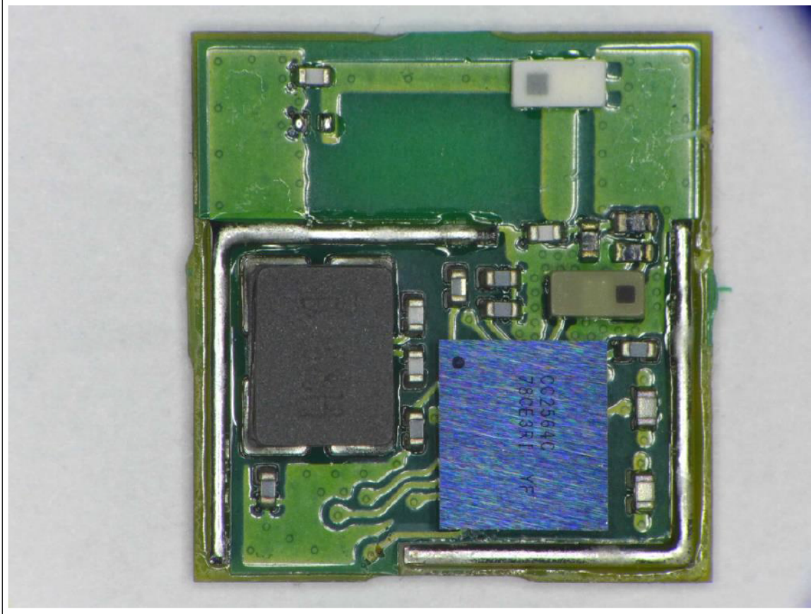
EUT PAN1326C2 without cover
