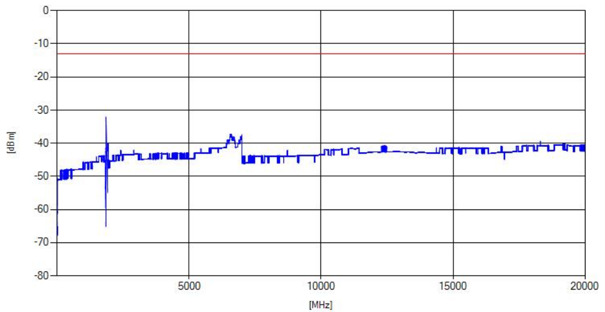
LTE eFDD 2 QPSK, Channel = low
