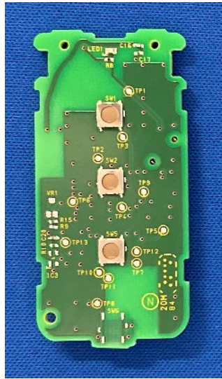
Figure 8.3 PCB assy (front view)
