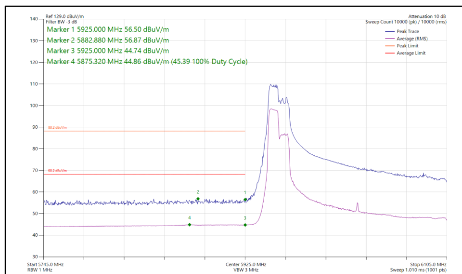
Figure 166 - 802.11ax HE160, RU 106-53P, SISO, Core 0 - 6025 MHz Band Edge Frequency 5925 MHz
