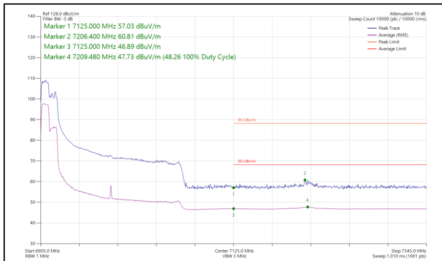
Figure 172 - 802.11ax HE160, RU 106-53P, SISO, Core 1 - 6985 MHz Band Edge Frequency 7125 MHz
