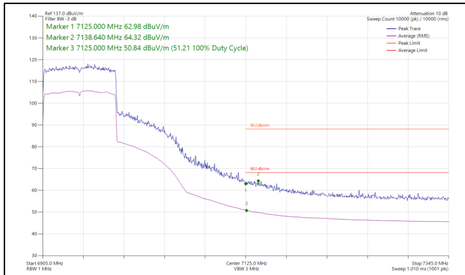
Figure 163 - 802.11ax HE80, SU, TxBF, Core 0 - Core 1 - 6945 MHz Band Edge Frequency 7125 MHz
