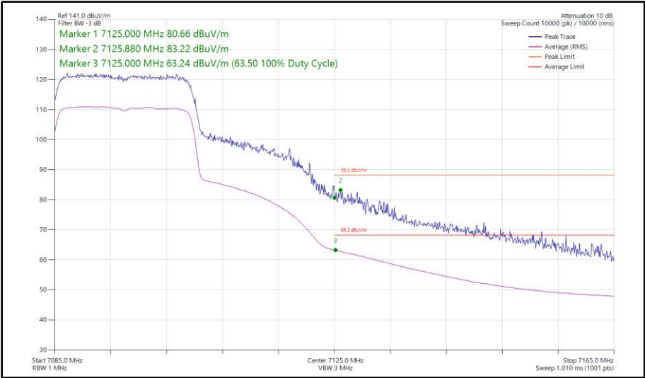
Figure 124 - 802.11ax HE20, SU, TxBF, Core 0 - Core 1 - 7095 MHz Band Edge Frequency 7125 MHz
