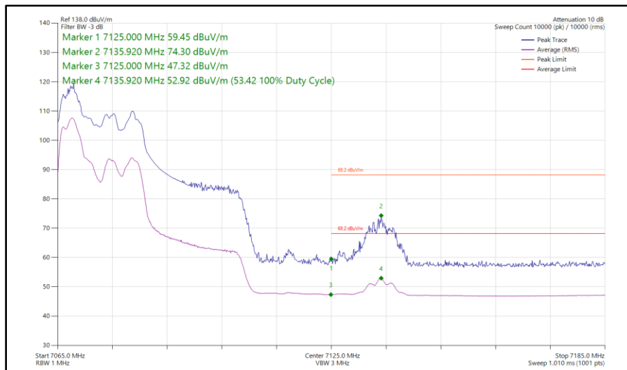
Figure 136 - 802.11ax HE40, RU 52-37, CDD, Core 0 - Core 1 - 7085 MHz Band Edge Frequency 7125 MHz
