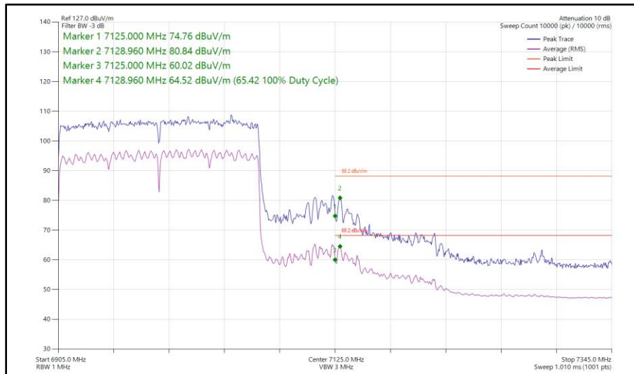
Figure 179 - 802.11ax HE160, SU, SDM, Core 0 - Core 1 - 6985 MHz Band Edge Frequency 7125 MHz
