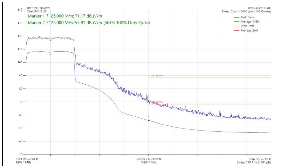
Figure 143 - 802.11ax HE40, SU, TxBF, Core 0 - Core 1 - 7045 MHz Band Edge Frequency 7125 MHz
