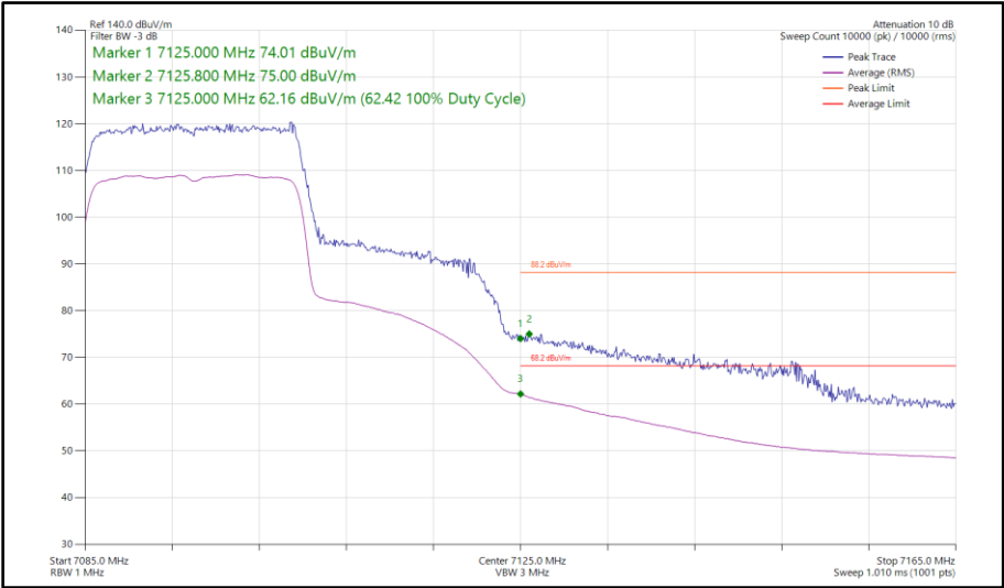
Figure 119 - 802.11ax HE20, SU, SDM, Core 0 - Core 1 - 7095 MHz Band Edge Frequency 7125 MHz
