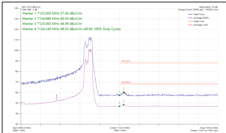
Figure 176 - 802.11ax HE160, RU 106-60S, CDD, Core 0 - Core 1 - 6985 MHz Band Edge Frequency 7125 MHz
