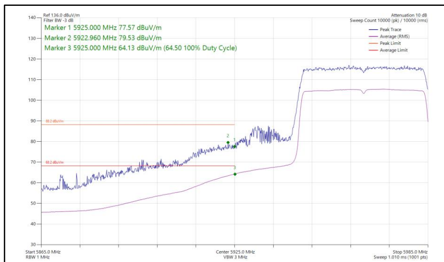
Figure 141 - 802.11ax HE40, SU, TxBF, Core 0 - Core 1 - 5965 MHz Band Edge Frequency 5925 MHz
