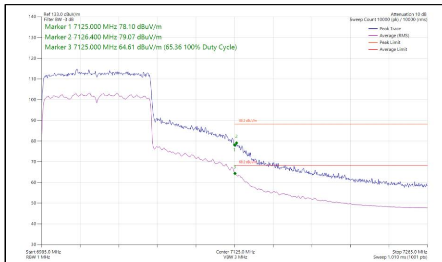
Figure 159 - 802.11ax HE80, SU, SDM, Core 0 - Core 1 - 7025 MHz Band Edge Frequency 7125 MHz
