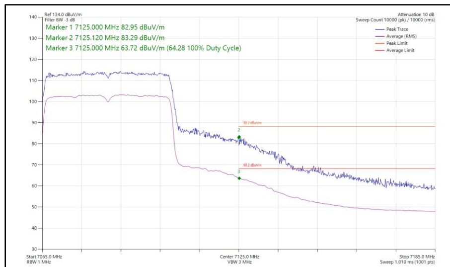
Figure 131 - 802.11ax HE40, SU, SISO, Core 1 - 7085 MHz Band Edge Frequency 7125 MHz
