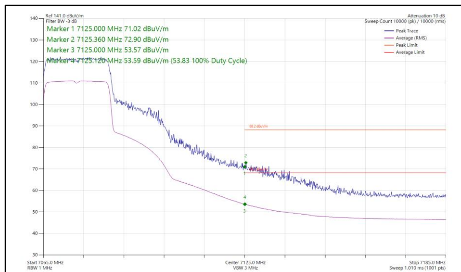
Figure 123 - 802.11ax HE20, SU, TxBF, Core 0 - Core 1 - 7075 MHz Band Edge Frequency 7125 MHz
