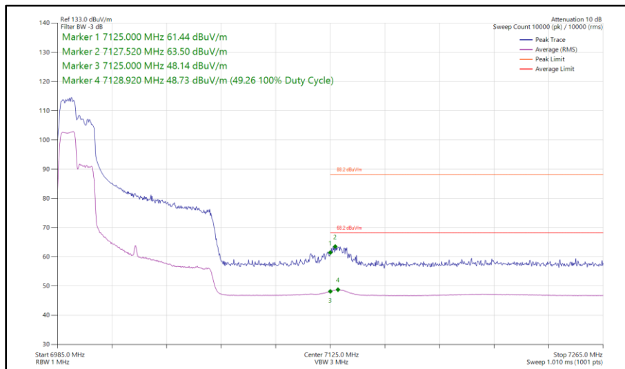
Figure 148 - 802.11ax HE80, RU 106-53, SISO, Core 0 - 7025 MHz Band Edge Frequency 7125 MHz
