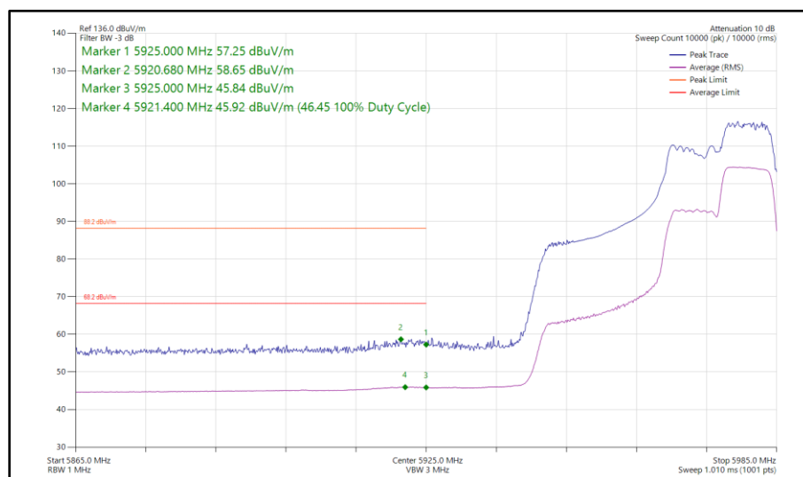
Figure 126 - 802.11ax HE40, RU 106-56, SISO, Core 0 - 5965 MHz Band Edge Frequency 5925 MHz
