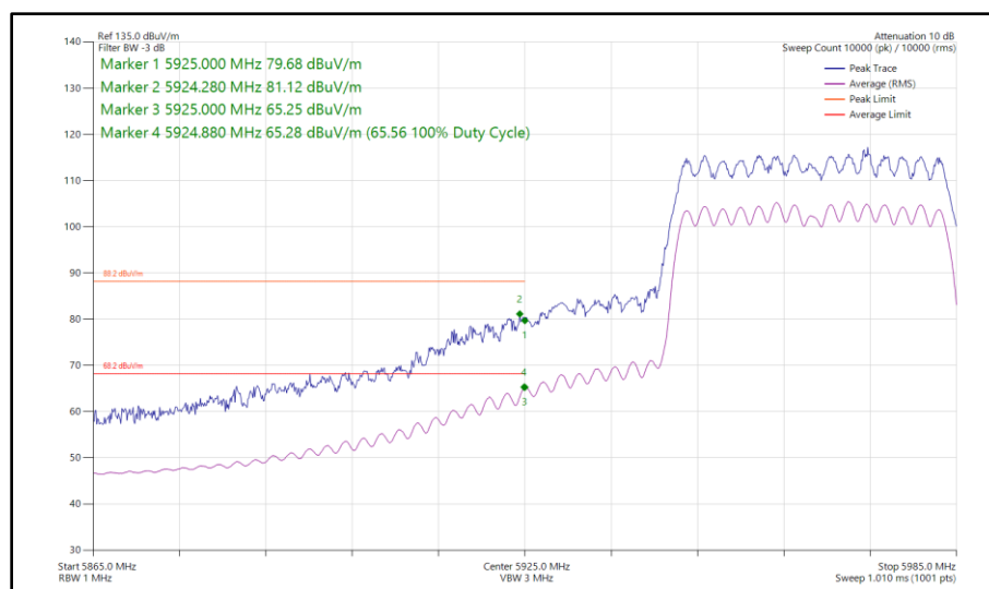
Figure 133 - 802.11ax HE40, SU, CDD, Core 0 - Core 1 - 5965 MHz Band Edge Frequency 5925 MHz
