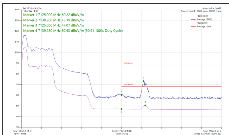
Figure 132 - 802.11ax HE40, RU 26-0, SISO, Core 1 - 7085 MHz Band Edge Frequency 7125 MHz
