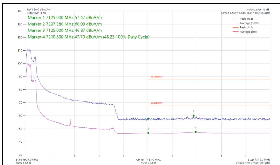
Figure 180 - 802.11ax HE160, RU 106-53P, SDM, Core 0 - Core 1 - 6985 MHz Band Edge Frequency 7125 MHz
