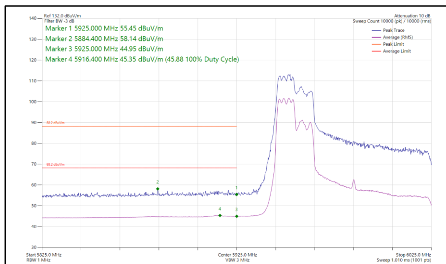
Figure 158 - 802.11ax HE80, RU 106-53, SDM, Core 0 - Core 1 - 5985 MHz Band Edge Frequency 5925 MHz
