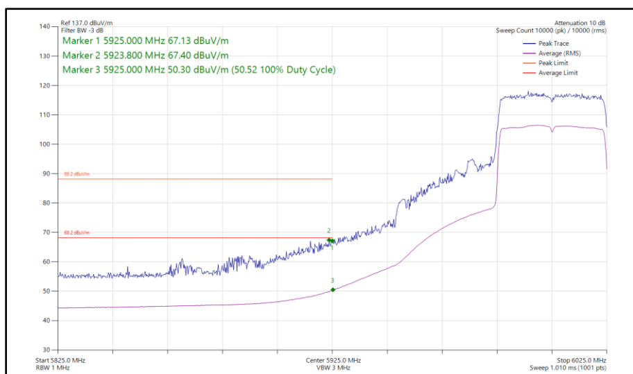
Figure 142 - 802.11ax HE40, SU, TxBF, Core 0 - Core 1 - 6005 MHz Band Edge Frequency 5925 MHz
