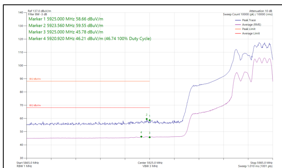
Figure 134 - 802.11ax HE40, RU 106-56, CDD, Core 0 - Core 1 - 5965 MHz Band Edge Frequency 5925 MHz
