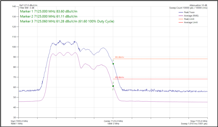
Figure 116 - 802.11ax HE20, RU 106-53, CDD, Core 0 - Core 1 - 7115 MHz Band Edge Frequency 7125 MHz
