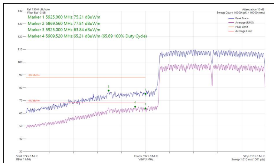
Figure 173 - 802.11ax HE160, SU, CDD, Core 0 - Core 1 - 6025 MHz Band Edge Frequency 5925 MHz
