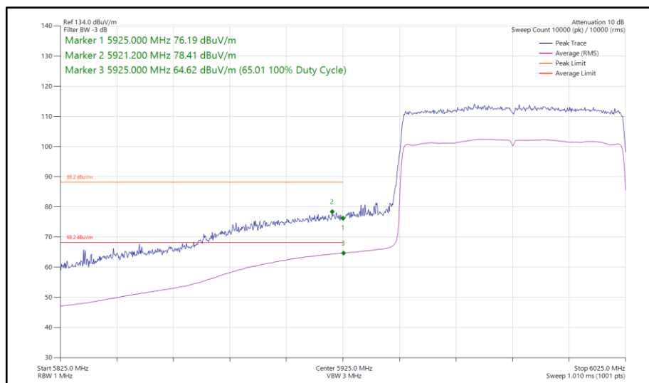
Figure 161 - 802.11ax HE80, SU, TxBF, Core 0 - Core 1 - 5985 MHz Band Edge Frequency 5925 MHz
