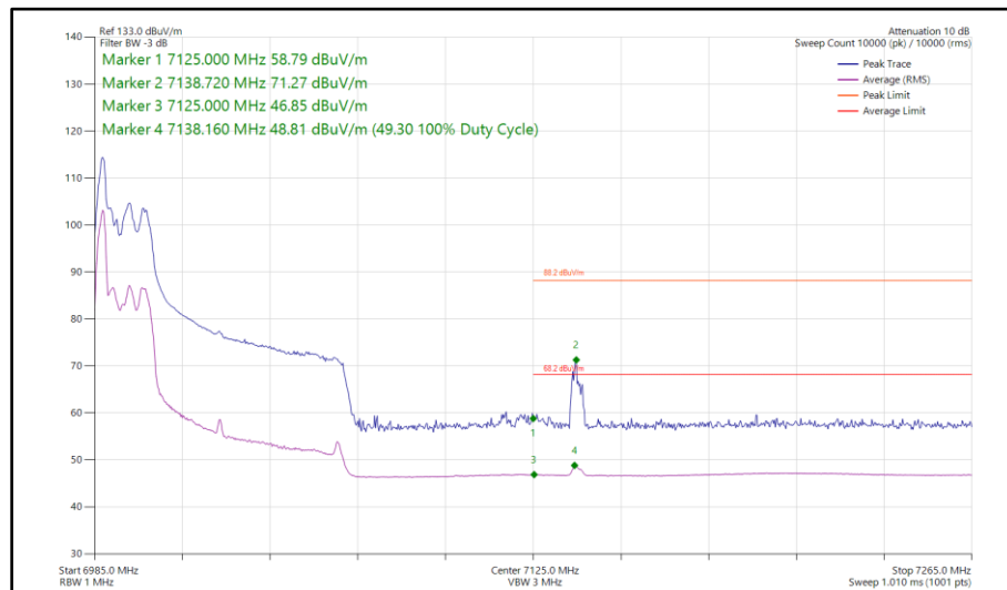
Figure 156 - 802.11ax HE80, RU 26-0, CDD, Core 0 - Core 1 - 7025 MHz Band Edge Frequency 7125 MHz
