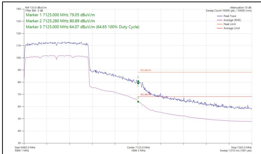
Figure 151 - 802.11ax HE80, SU, SISO, Core 1 - 7025 MHz Band Edge Frequency 7125 MHz
