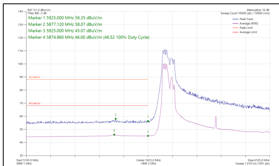
Figure 174 - 802.11ax HE160, RU 106-53P, CDD, Core 0 - Core 1 - 6025 MHz Band Edge Frequency 5925 MHz
