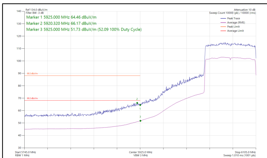
Figure 162 - 802.11ax HE80, SU, TxBF, Core 0 - Core 1 - 6065 MHz Band Edge Frequency 5925 MHz
