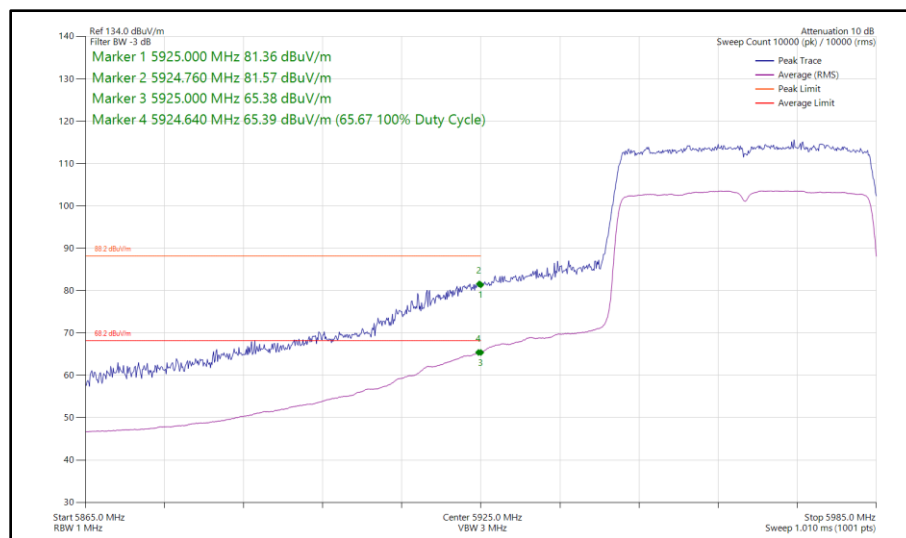
Figure 125 - 802.11ax HE40, SU, SISO, Core 0 - 5965 MHz Band Edge Frequency 5925 MHz
