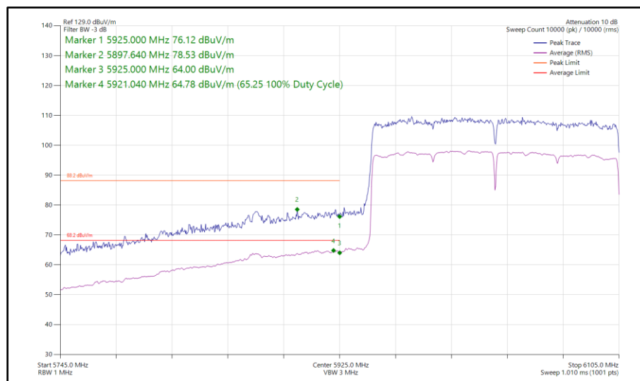
Figure 169 - 802.11ax HE160, SU, SISO, Core 1 - 6025 MHz Band Edge Frequency 5925 MHz
