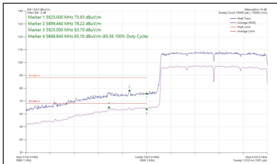
Figure 177 - 802.11ax HE160, SU, SDM, Core 0 - Core 1 - 6025 MHz Band Edge Frequency 5925 MHz
