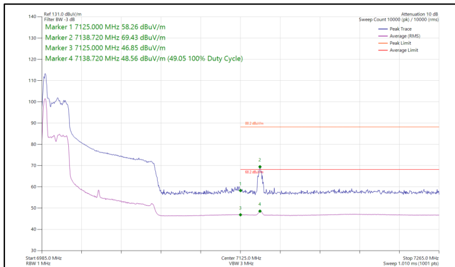
Figure 152 - 802.11ax HE80, RU 26-0, SISO, Core 1 - 7025 MHz Band Edge Frequency 7125 MHz
