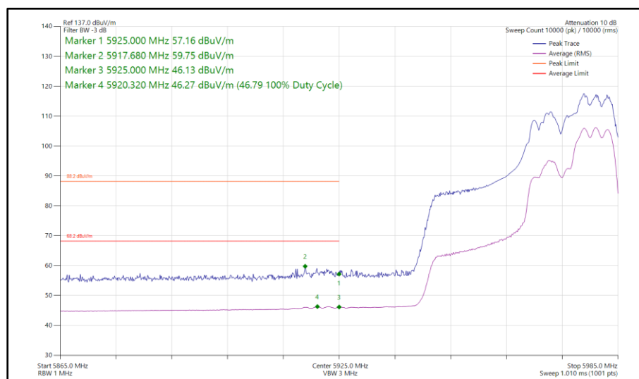
Figure 138 - 802.11ax HE40, RU 106-56, SDM, Core 0 - Core 1 - 5965 MHz Band Edge Frequency 5925 MHz
