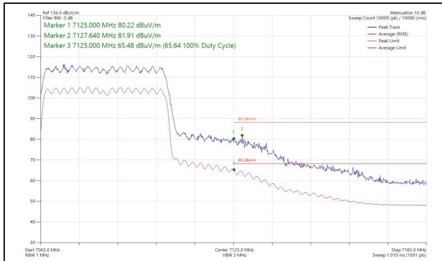
Figure 135 - 802.11ax HE40, SU, CDD, Core 0 - Core 1 - 7085 MHz Band Edge Frequency 7125 MHz
