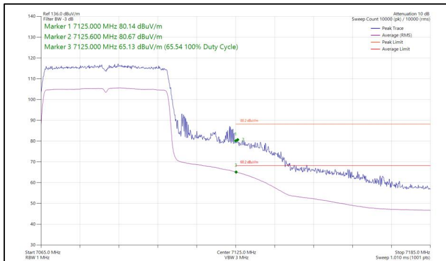
Figure 144 - 802.11ax HE40, SU, TxBF, Core 0 - Core 1 - 7085 MHz Band Edge Frequency 7125 MHz
