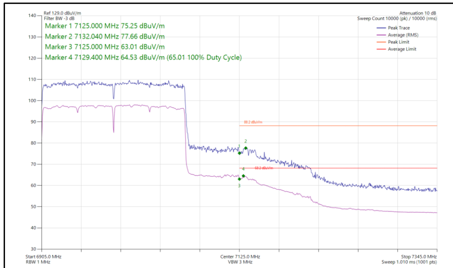
Figure 167 - 802.11ax HE160, SU, SISO, Core 0 - 6985 MHz Band Edge Frequency 7125 MHz
