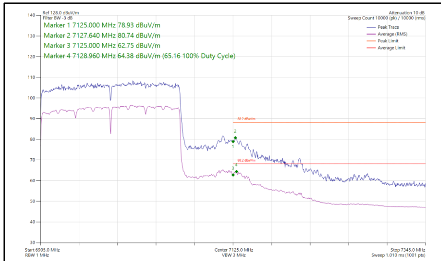
Figure 171 - 802.11ax HE160, SU, SISO, Core 1 - 6985 MHz Band Edge Frequency 7125 MHz
