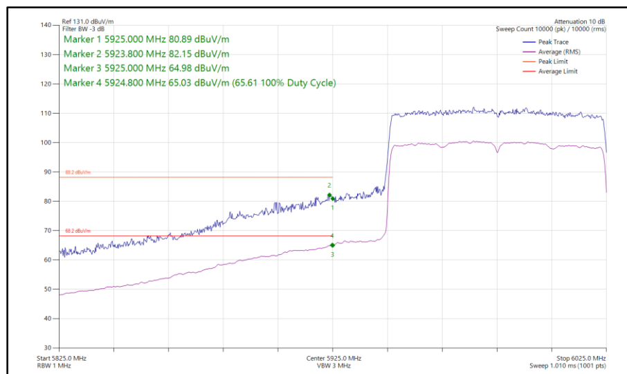
Figure 149 - 802.11ax HE80, SU, SISO, Core 1 - 5985 MHz Band Edge Frequency 5925 MHz
