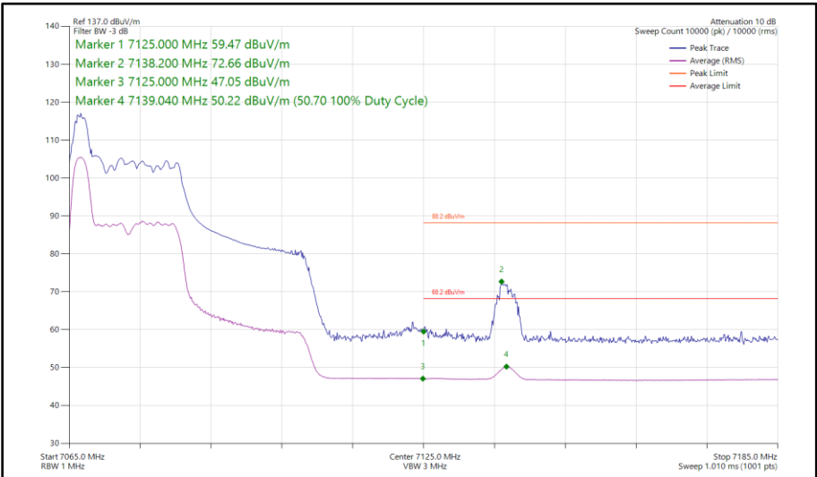
Figure 128 - 802.11ax HE40, RU 26-0, SISO, Core 0 - 7085 MHz Band Edge Frequency 7125 MHz
