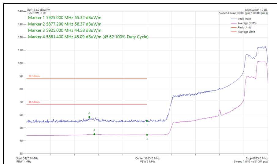
Figure 150 - 802.11ax HE80, RU 106-60, SISO, Core 1 - 5985 MHz Band Edge Frequency 5925 MHz
