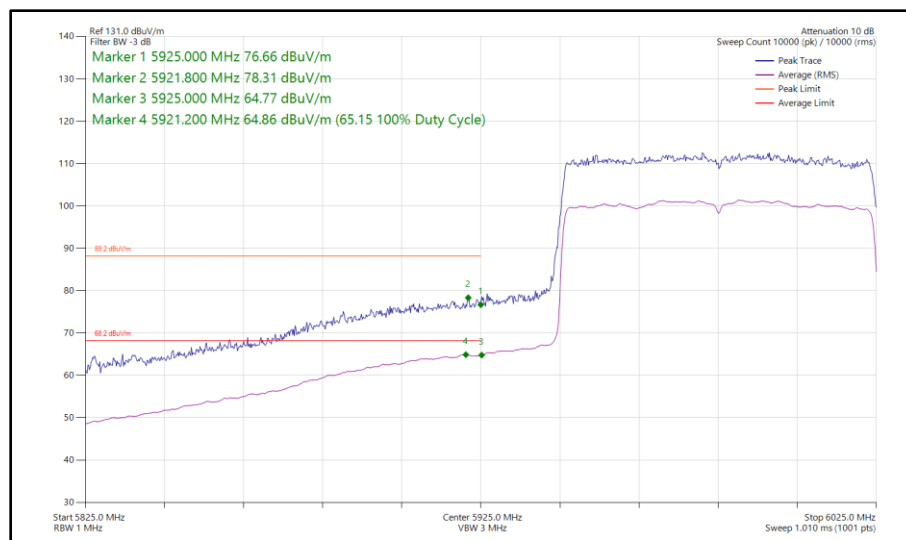
Figure 157 - 802.11ax HE80, SU, SDM, Core 0 - Core 1 - 5985 MHz Band Edge Frequency 5925 MHz
