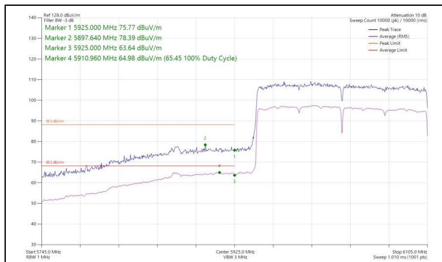
Figure 165 - 802.11ax HE160, SU, SISO, Core 0 - 6025 MHz Band Edge Frequency 5925 MHz
