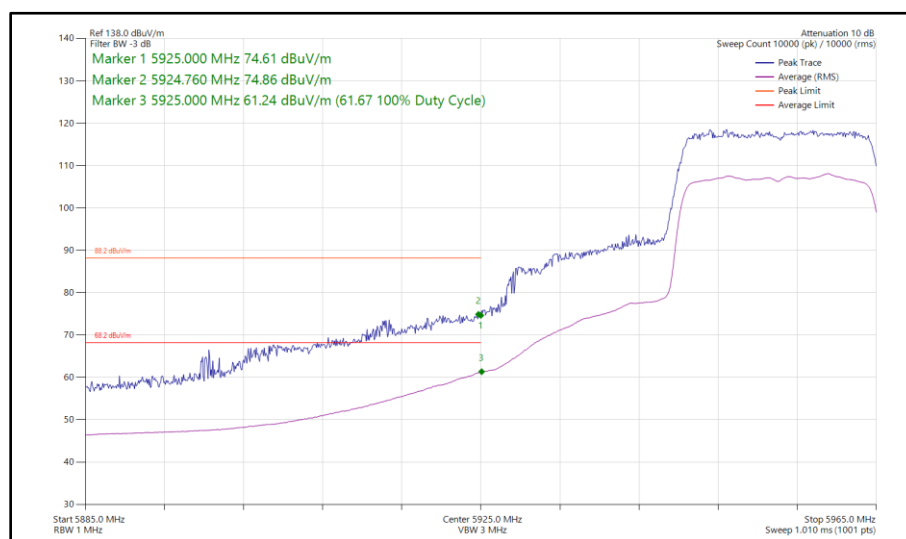
Figure 117 - 802.11ax HE20, SU, SDM, Core 0 - Core 1 - 5955 MHz Band Edge Frequency 5925 MHz
