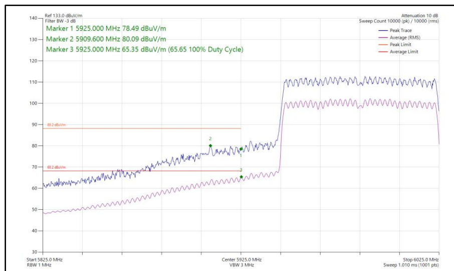
Figure 153 - 802.11ax HE80, SU, CDD, Core 0 - Core 1 - 5985 MHz Band Edge Frequency 5925 MHz
