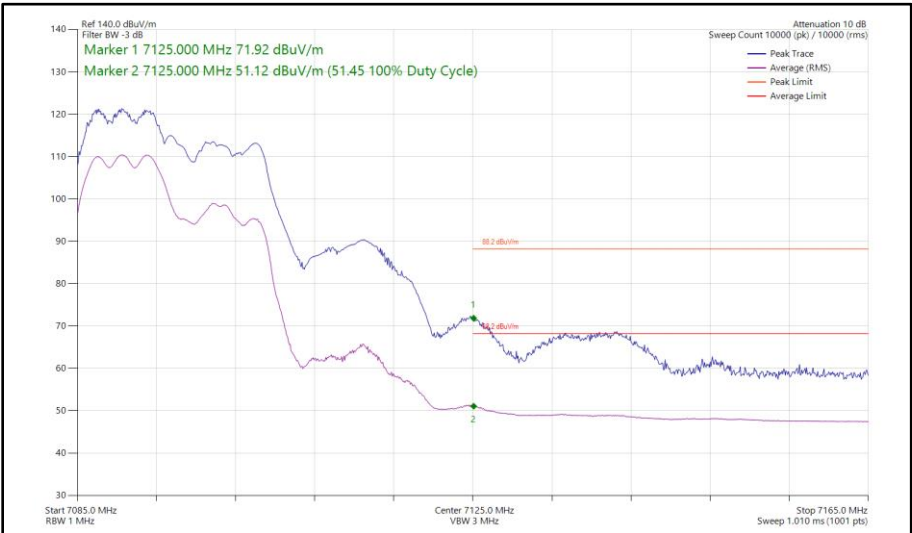
Figure 115 - 802.11ax HE20, RU 106-53, CDD, Core 0 - Core 1 - 7095 MHz Band Edge Frequency 7125 MHz
