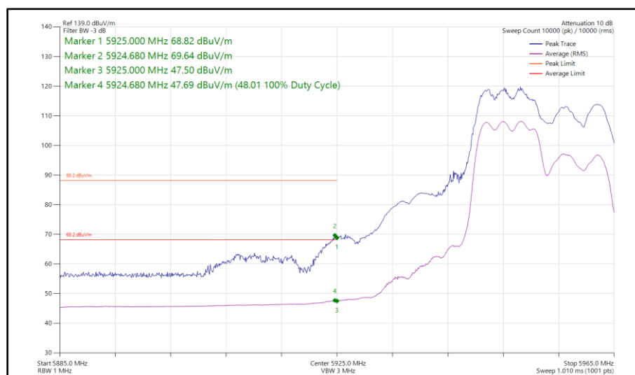
Figure 118 - 802.11ax HE20, RU 106-53, SDM, Core 0 - Core 1 - 5955 MHz Band Edge Frequency 5925 MHz
