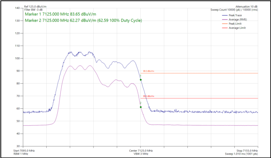
Figure 121 - 802.11ax HE20, RU 106-53, SDM, Core 0 - Core 1 - 7115 MHz Band Edge Frequency 7125 MHz
