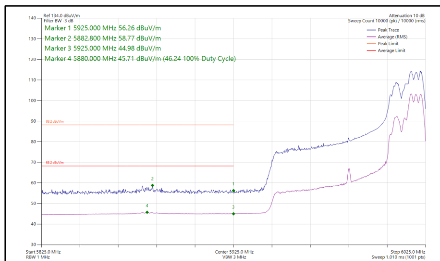
Figure 154 - 802.11ax HE80, RU 106-60, CDD, Core 0 - Core 1 - 5985 MHz Band Edge Frequency 5925 MHz
