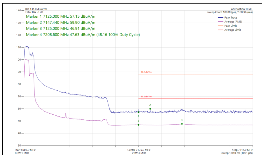
Figure 168 - 802.11ax HE160, RU 106-53P, SISO, Core 0 - 6985 MHz Band Edge Frequency 7125 MHz
