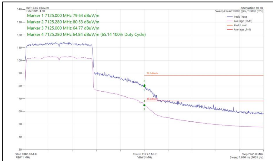
Figure 147 - 802.11ax HE80, SU, SISO, Core 0 - 7025 MHz Band Edge Frequency 7125 MHz
