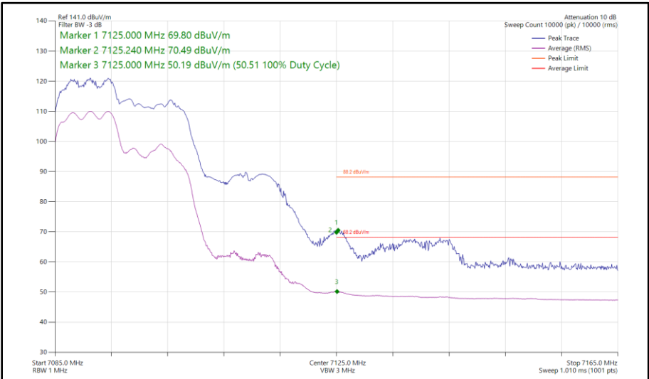
Figure 120 - 802.11ax HE20, RU 106-53, SDM, Core 0 - Core 1 - 7095 MHz Band Edge Frequency 7125 MHz
