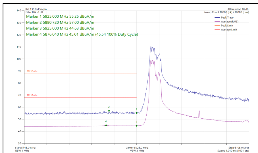
Figure 178 - 802.11ax HE160, RU 106-53P, SDM, Core 0 - Core 1 - 6025 MHz Band Edge Frequency 5925 MHz
