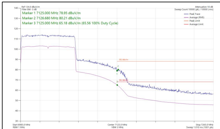
Figure 164 - 802.11ax HE80, SU, TxBF, Core 0 - Core 1 - 7025 MHz Band Edge Frequency 7125 MHz
