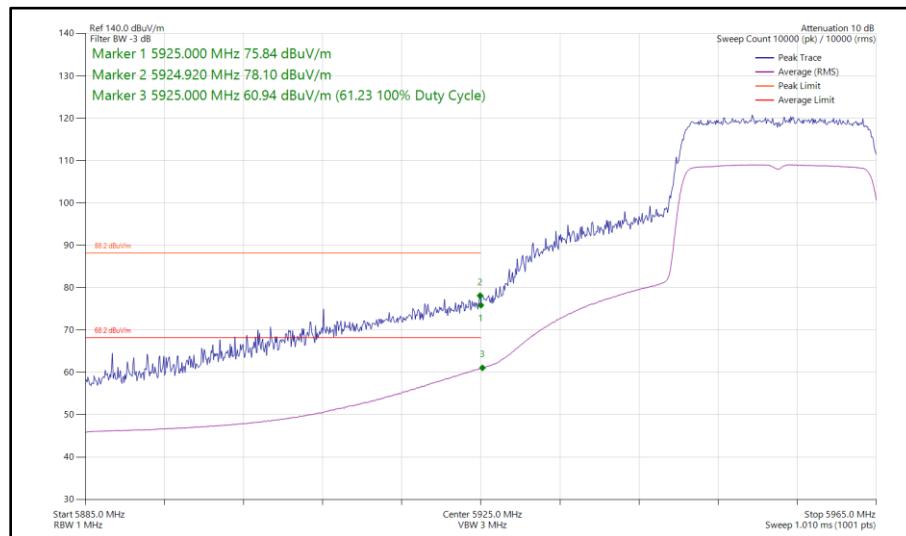
Figure 122 - 802.11ax HE20, SU, TxBF, Core 0 - Core 1 - 5955 MHz Band Edge Frequency 5925 MHz
