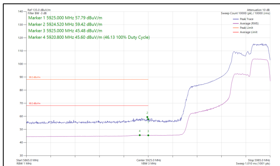
Figure 130 - 802.11ax HE40, RU 106-56, SISO, Core 1 - 5965 MHz Band Edge Frequency 5925 MHz
