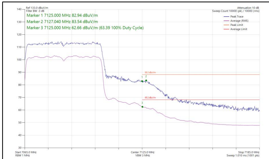
Figure 139 - 802.11ax HE40, SU, SDM, Core 0 - Core 1 - 7085 MHz Band Edge Frequency 7125 MHz
