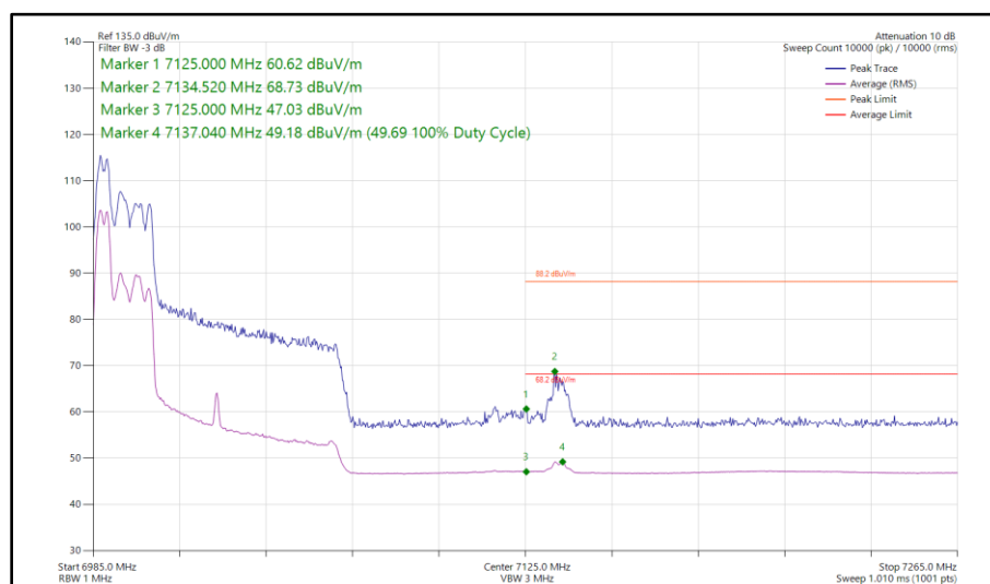
Figure 160 - 802.11ax HE80, RU 52-37, SDM, Core 0 - Core 1 - 7025 MHz Band Edge Frequency 7125 MHz
