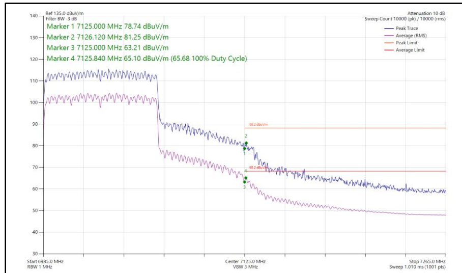
Figure 155 - 802.11ax HE80, SU, CDD, Core 0 - Core 1 - 7025 MHz Band Edge Frequency 7125 MHz
