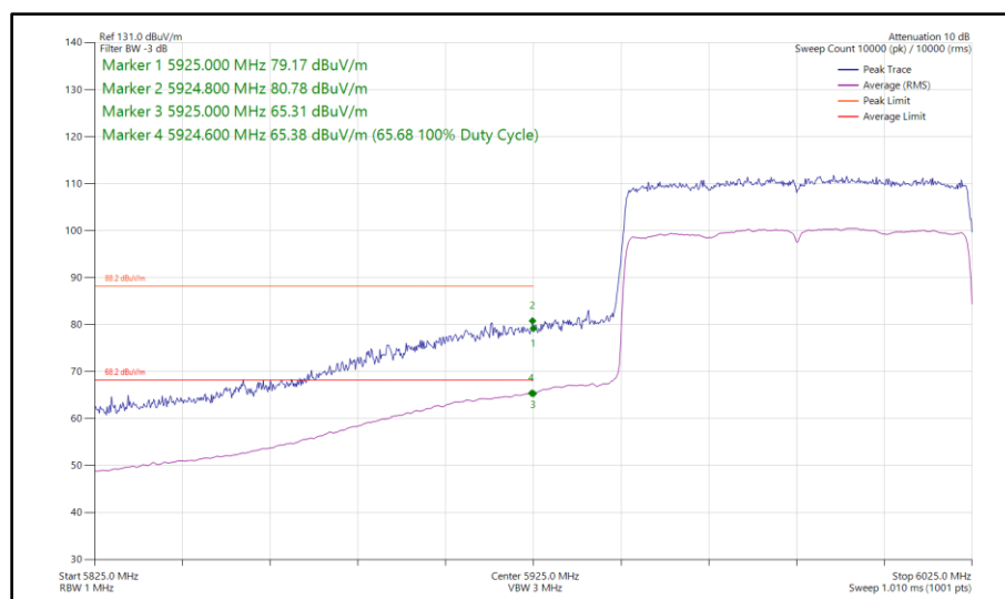
Figure 145 - 802.11ax HE80, SU, SISO, Core 0 - 5985 MHz Band Edge Frequency 5925 MHz
