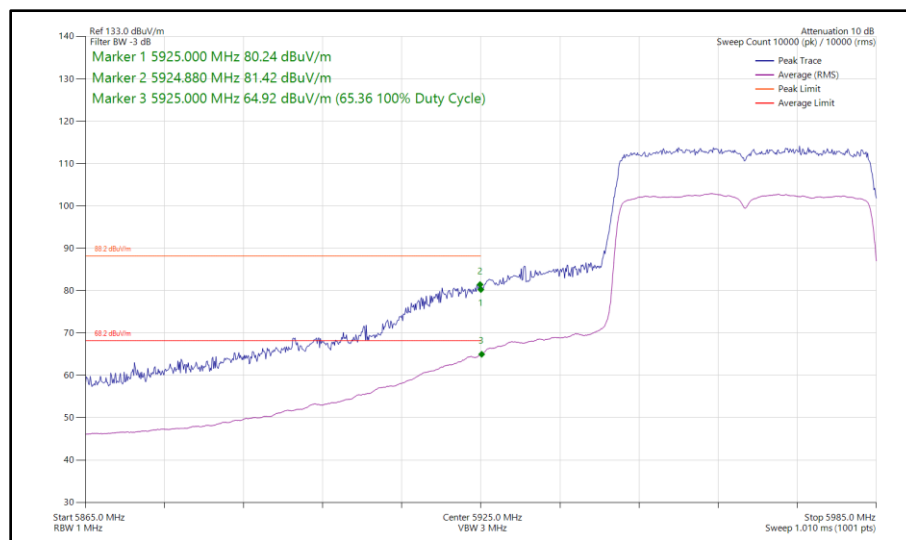
Figure 137 - 802.11ax HE40, SU, SDM, Core 0 - Core 1 - 5965 MHz Band Edge Frequency 5925 MHz
