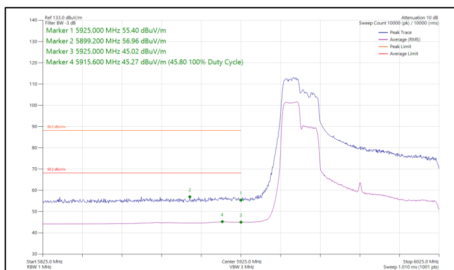
Figure 146 - 802.11ax HE80, RU 106-53, SISO, Core 0 - 5985 MHz Band Edge Frequency 5925 MHz
