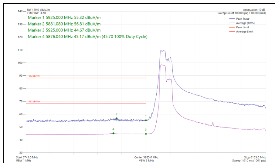
Figure 170 - 802.11ax HE160, RU 106-53P, SISO, Core 1 - 6025 MHz Band Edge Frequency 5925 MHz
