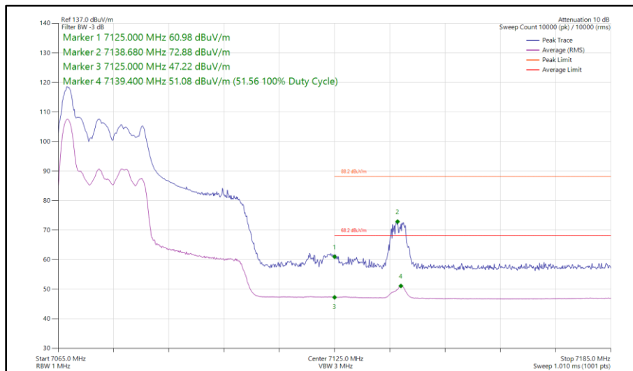
Figure 140 - 802.11ax HE40, RU 26-0, SDM, Core 0 - Core 1 - 7085 MHz Band Edge Frequency 7125 MHz
