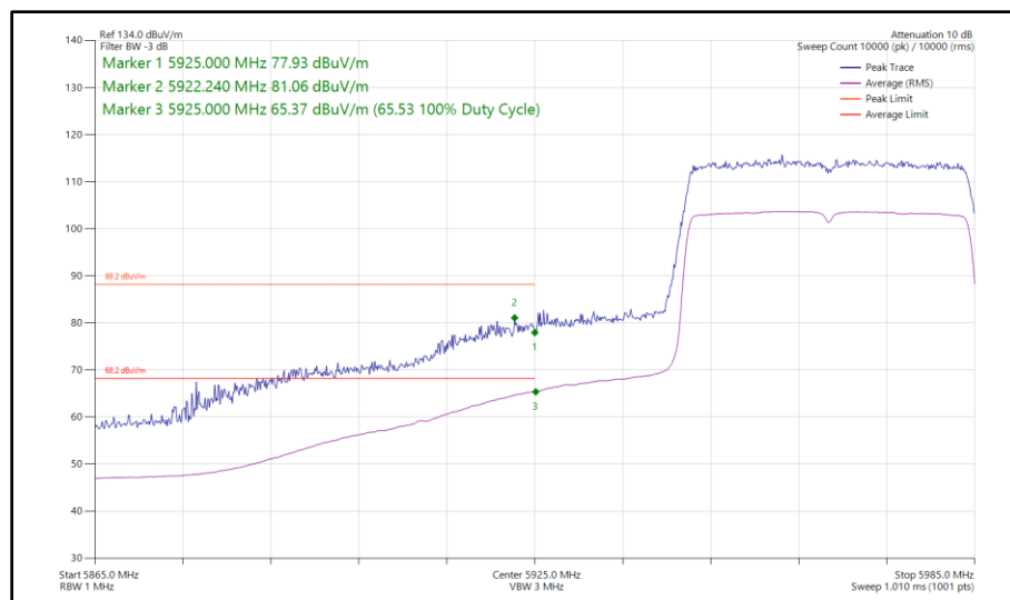
Figure 129 - 802.11ax HE40, SU, SISO, Core 1 - 5965 MHz Band Edge Frequency 5925 MHz
