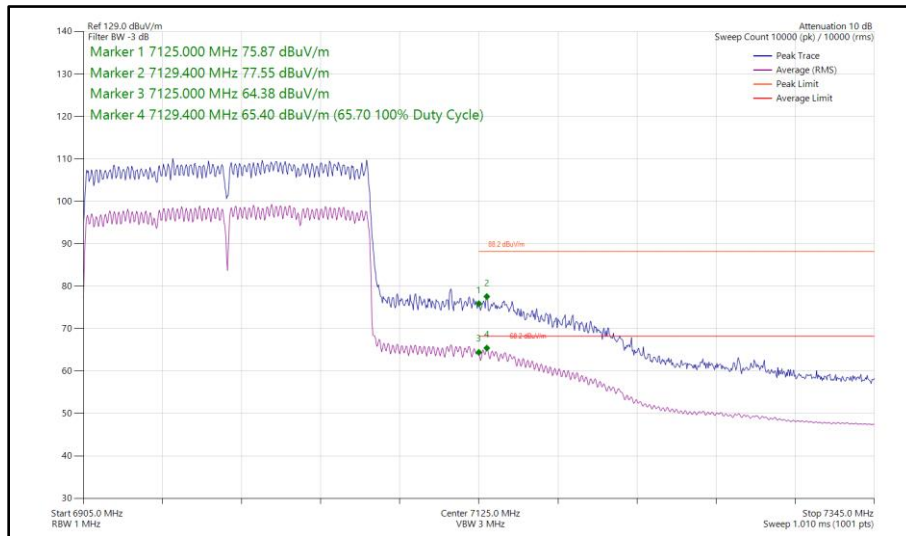
Figure 175 - 802.11ax HE160, SU, CDD, Core 0 - Core 1 - 6985 MHz Band Edge Frequency 7125 MHz
