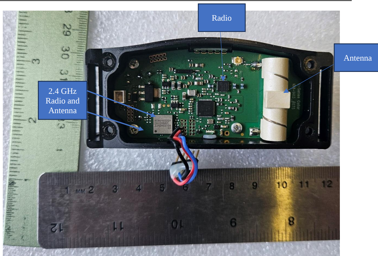
Figure 2. Main PCB Front and Antenna (300-3444)
