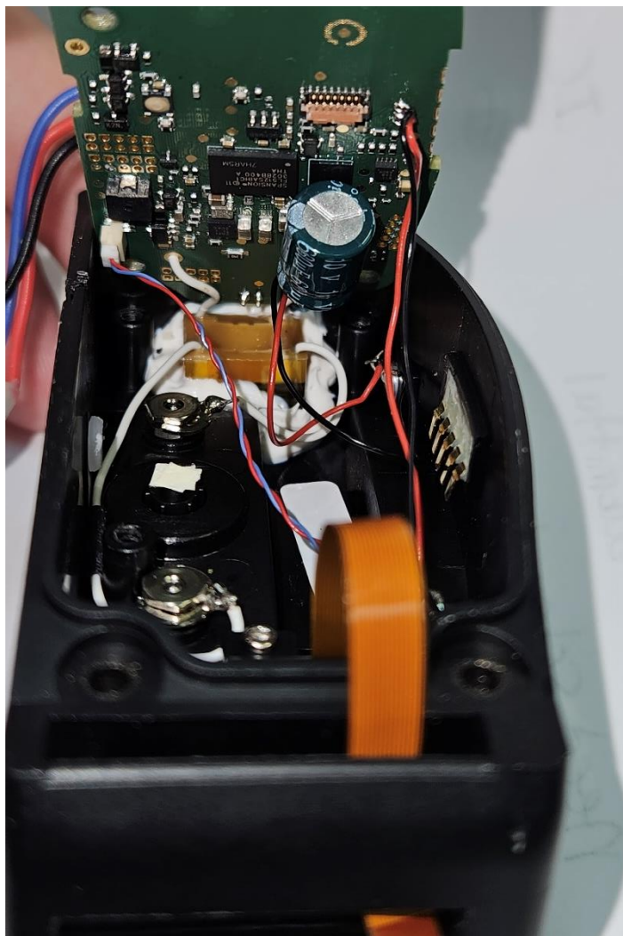
Figure 7. Main PCB Back (300-3446)
