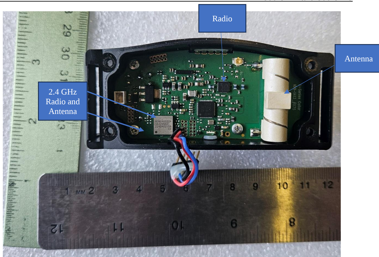
Figure 6. Main PCB Front and Antenna (300-3446)
