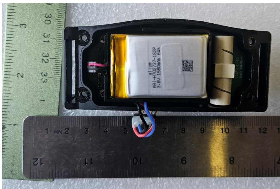
Figure 8. Battery (300-3446)
