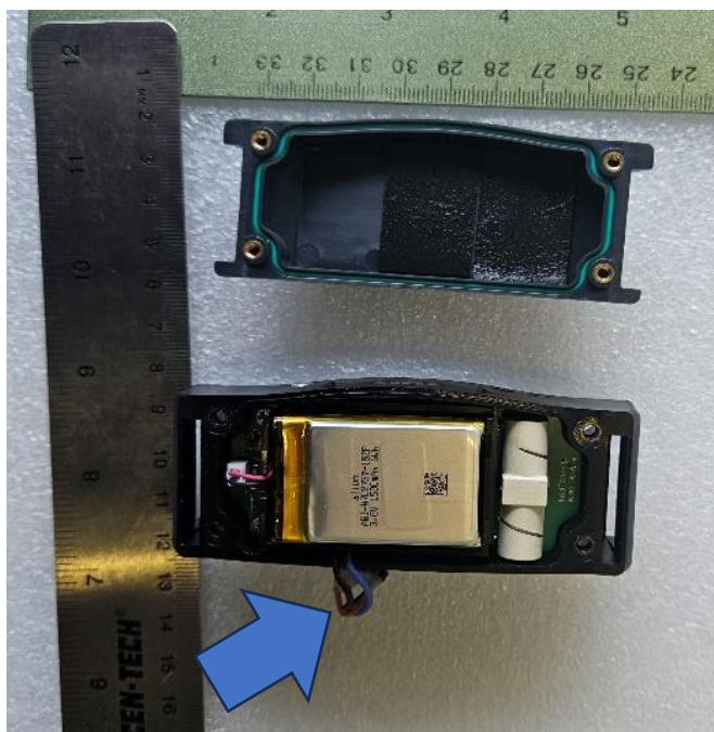
Figure 5. Back Cover Removed (300-3446)
