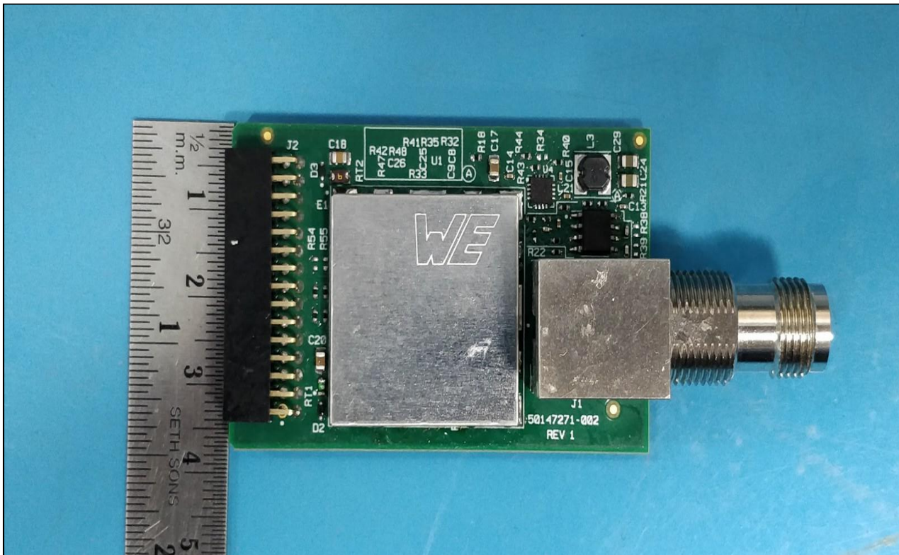
Photo 2: PCB Dimensional View
