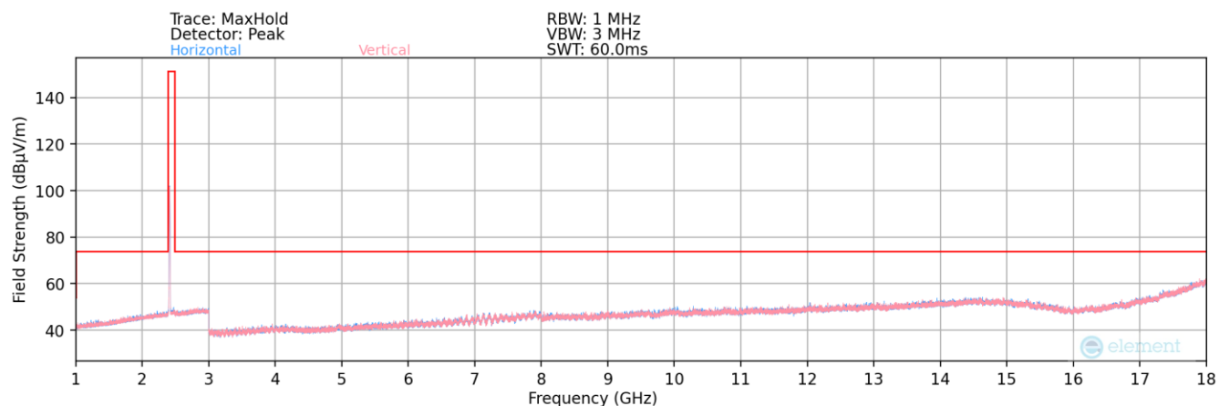
Plot 7-141. Radiated Spurious Plot above 1GHz MIMO (802.11b – Ch. 1)
