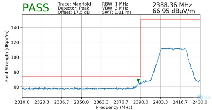
Plot 7-162. Radiated Restricted Lower Band Edge Measurement MIMO (Peak)
