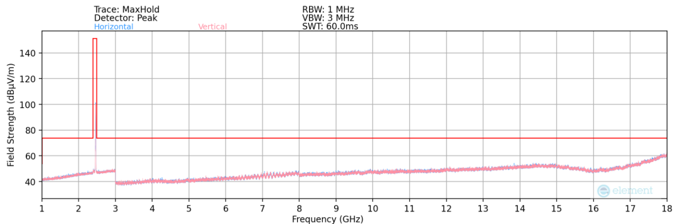
Plot 7-143. Radiated Spurious Plot above 1GHz MIMO (802.11b – Ch. 11)
