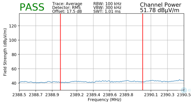
Plot 7-161. Radiated Restricted Lower Band Edge Measurement MIMO (Average)
