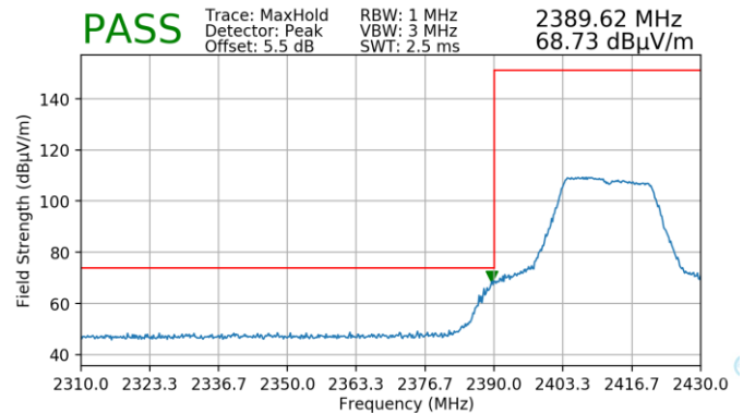
Plot 7-154. Radiated Restricted Lower Band Edge Measurement SISO ANT2 (Peak)
