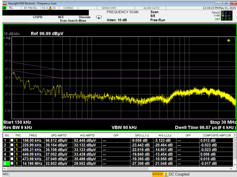
Plot 7-171. Line Conducted Plot with 802.11b (L1)_M2
