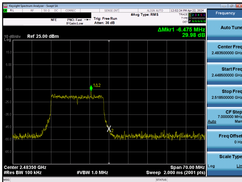
Plot 7-121. Band Edge Plot MIMO ANT2 (802.11ax/be (2.4GHz) – Ch. 13)
