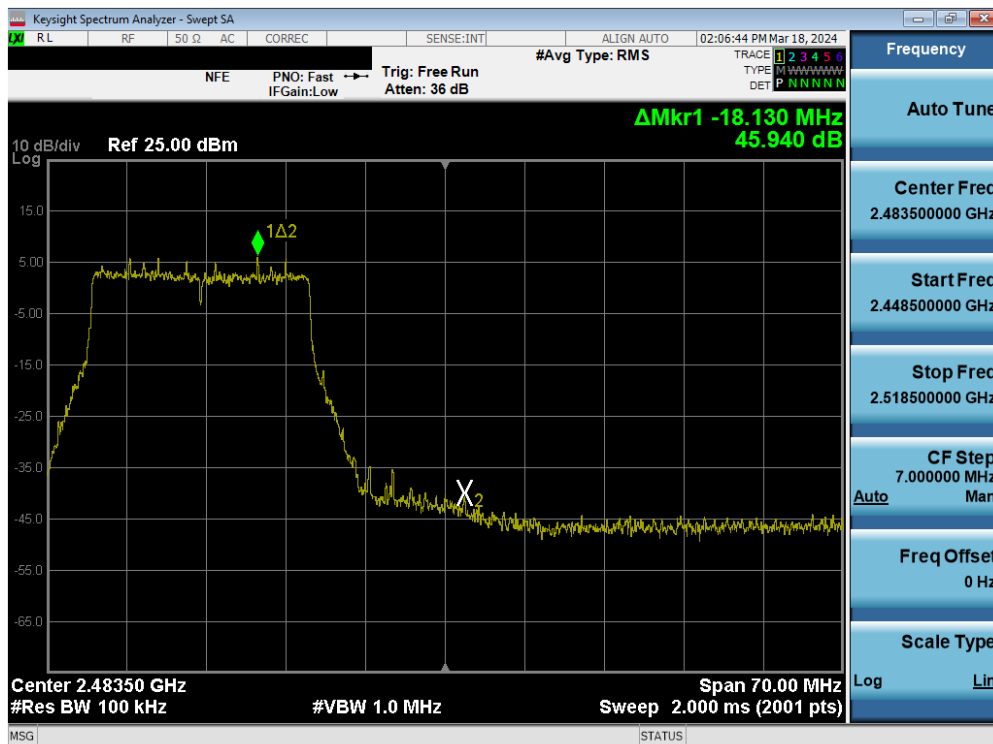
Plot 7-119. Band Edge Plot MIMO ANT2 (802.11ax/be (2.4GHz) – Ch. 11)
