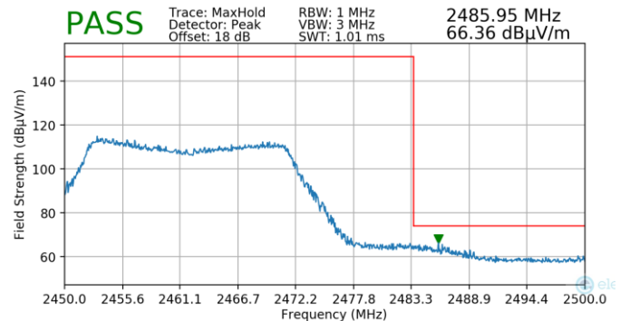
Plot 7-164. Radiated Restricted Upper Band Edge Measurement MIMO (Peak)
