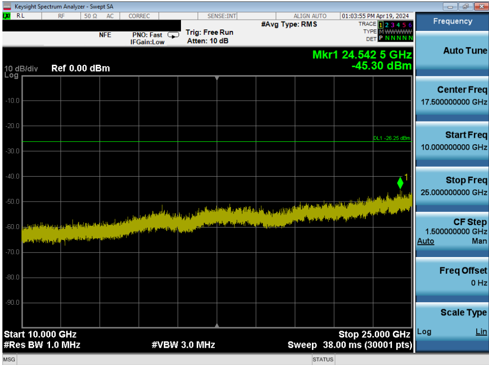
Plot 7-127. Conducted Spurious Plot SISO ANT2 (802.11b – Ch. 11)
