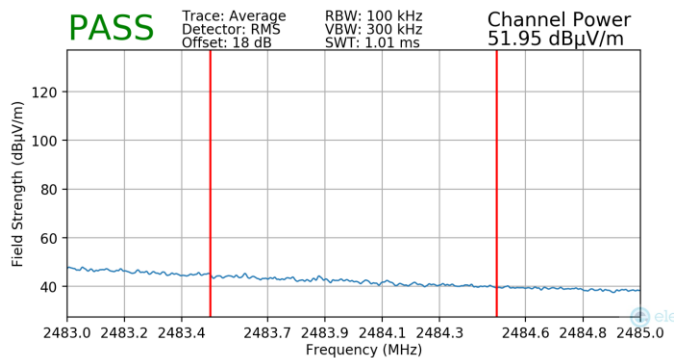
Plot 7-167. Radiated Restricted Upper Band Edge Measurement MIMO (Average)
