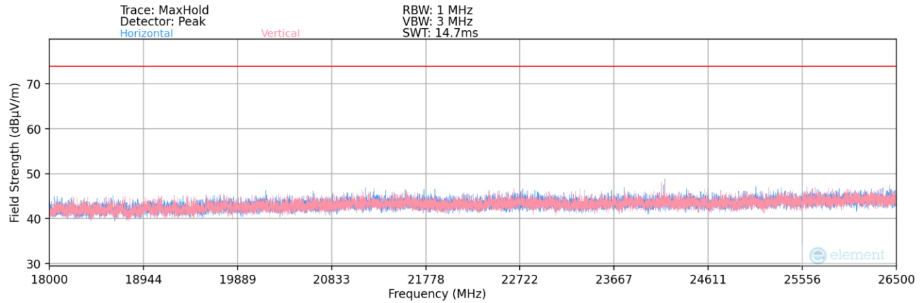
Plot 7-151. Radiated Spurious Plot 18GHz – 26.5GHz (2.4GHz –6GHz)
