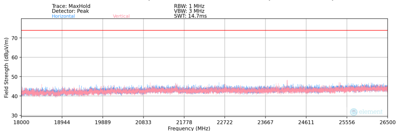
Plot 7-144. Radiated Spurious Plot above 18GHz MIMO
