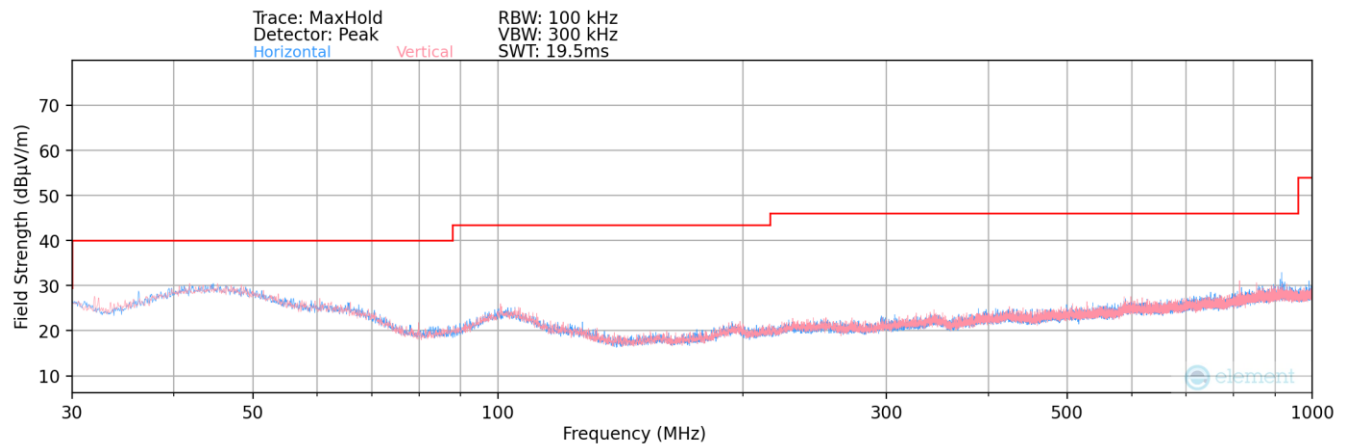
Plot 7-149. Radiated Spurious Plot below 1GHz (2.4GHz –6GHz)
