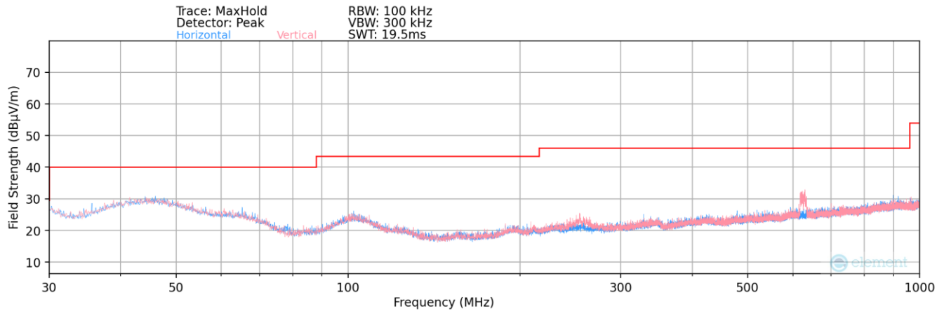
Plot 7-145. Radiated Spurious Plot below 1GHz (2.4GHz – 5GHz)
