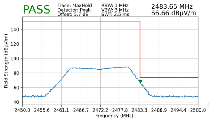
Plot 7-160. Radiated Restricted Upper Band Edge Measurement SISO ANT2 (Peak)
