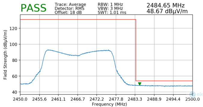
Plot 7-165. Radiated Restricted Upper Band Edge Measurement MIMO (Average)
