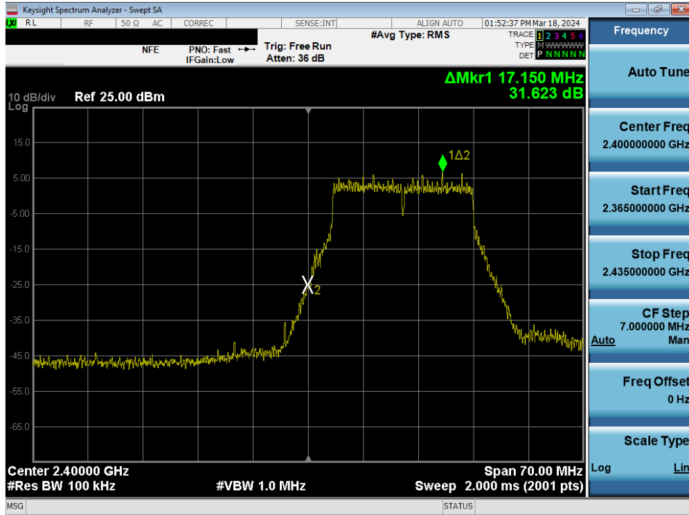
Plot 7-114. Band Edge Plot MIMO ANT2 (802.11n (2.4GHz) – Ch. 1)
