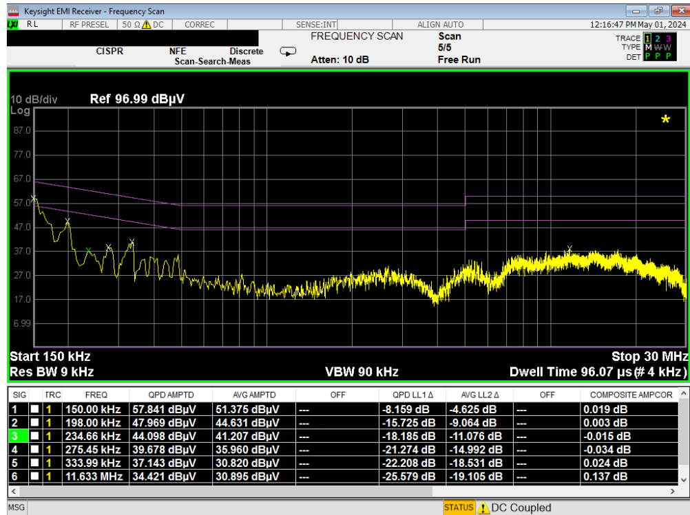
Plot 7-172. Line Conducted Plot with 802.11b (N)_M2
