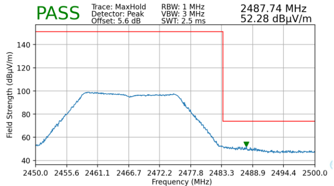
Plot 7-158. Radiated Restricted Upper Band Edge Measurement SISO ANT2 (Peak)
