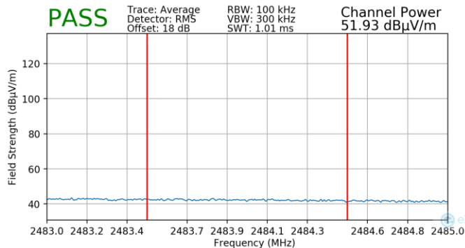
Plot 7-163. Radiated Restricted Upper Band Edge Measurement MIMO (Average)
