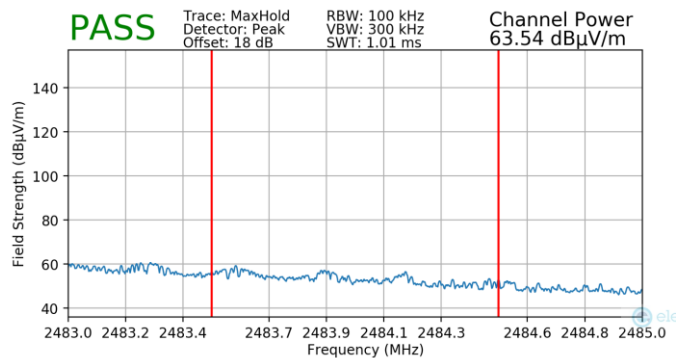
Plot 7-168. Radiated Restricted Upper Band Edge Measurement MIMO (Peak)
