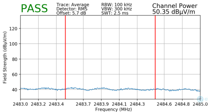
Plot 7-155. Radiated Restricted Upper Band Edge Measurement SISO ANT2 (Average)
