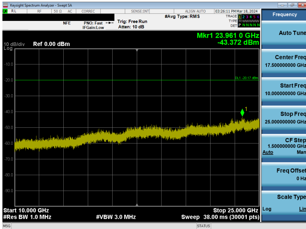
Plot 7-137. Conducted Spurious Plot MIMO ANT2 (802.11b – Ch. 6)
