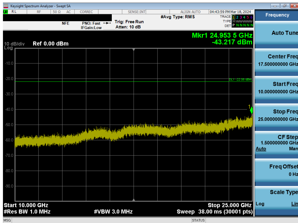
Plot 7-129. Conducted Spurious Plot MIMO ANT1 (802.11b – Ch. 1)
