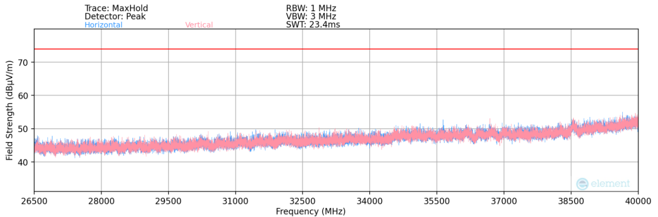
Plot 7-148. Radiated Spurious Plot above 26.5GHz (2.4GHz – 5GHz)
