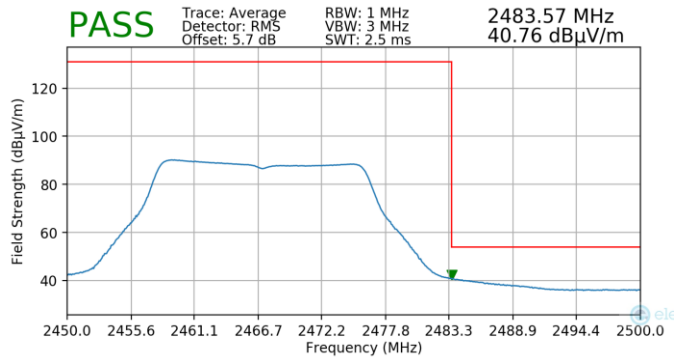
Plot 7-157. Radiated Restricted Upper Band Edge Measurement SISO ANT2 (Average)
