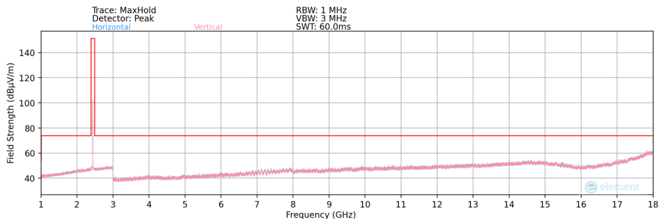
Plot 7-142. Radiated Spurious Plot above 1GHz MIMO (802.11b – Ch. 6)
