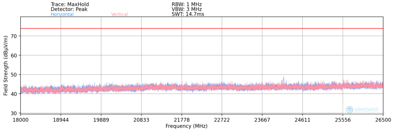
Plot 7-147. Radiated Spurious Plot 18GHz – 26.5GHz (2.4GHz – 5GHz)
