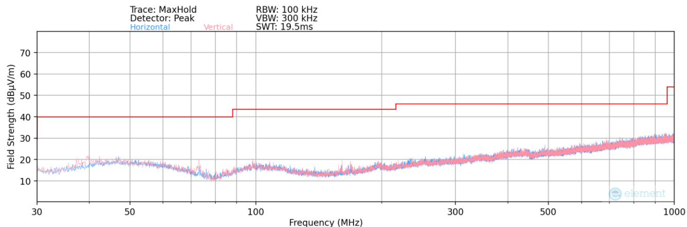
Plot 7-140. Radiated Spurious Plot below 1GHz MIMO
