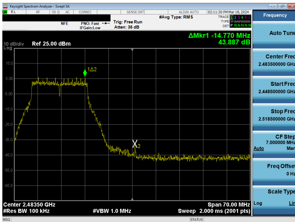
Plot 7-111. Band Edge Plot MIMO ANT2 (802.11g - Ch. 11)
