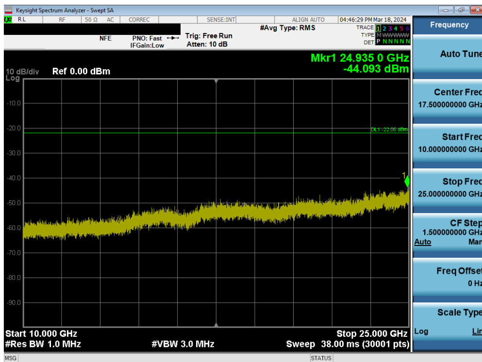
Plot 7-131. Conducted Spurious Plot MIMO ANT1 (802.11b – Ch. 6)
