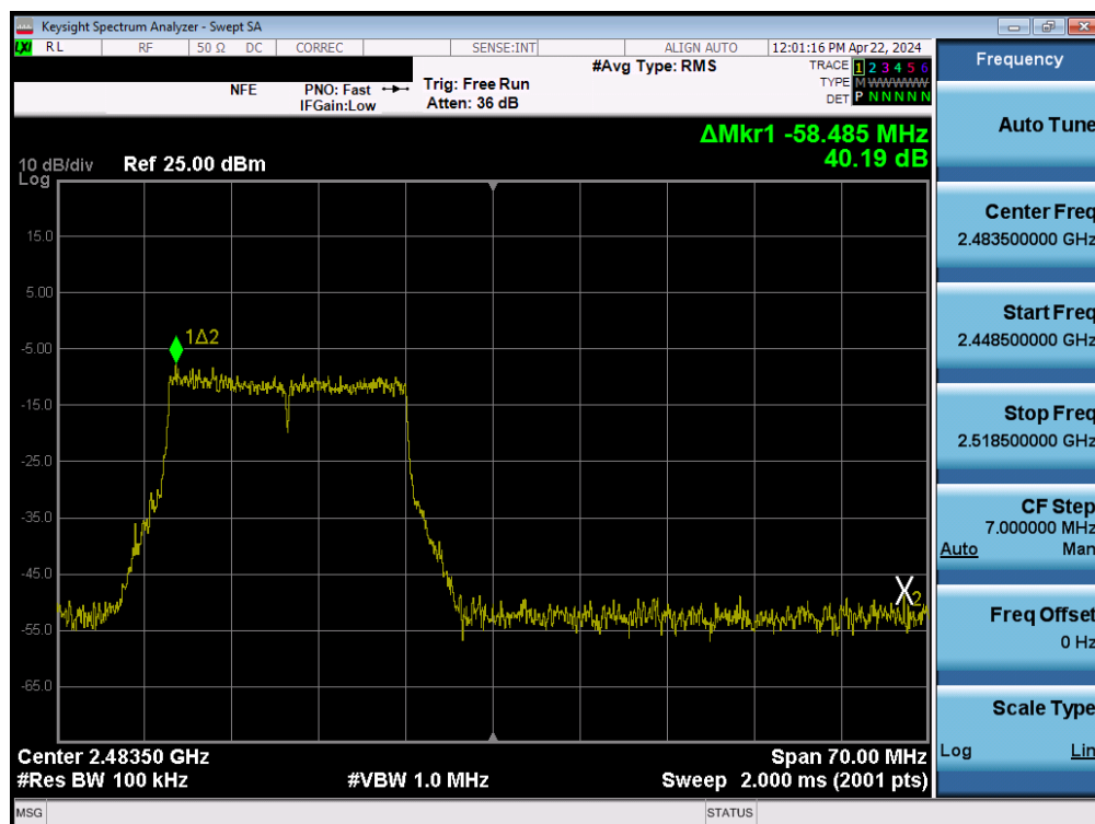
Plot 7-120. Band Edge Plot MIMO ANT2 (802.11ax/be (2.4GHz) – Ch. 12)
