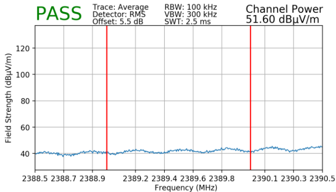
Plot 7-153. Radiated Restricted Lower Band Edge Measurement SISO ANT2 (Average)
