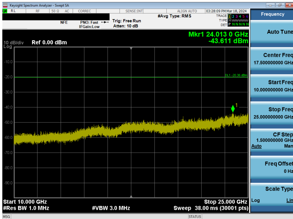
Plot 7-139. Conducted Spurious Plot MIMO ANT2 (802.11b – Ch. 11)
