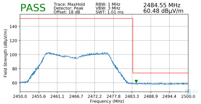
Plot 7-166. Radiated Restricted Upper Band Edge Measurement MIMO (Peak)
