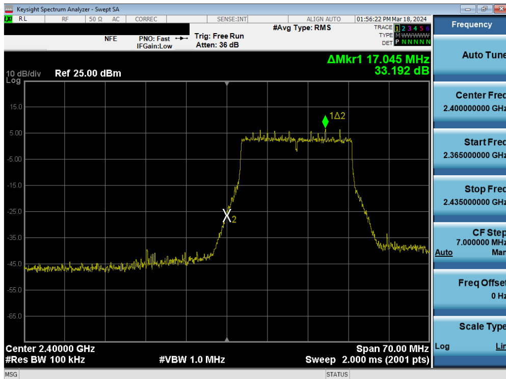
Plot 7-118. Band Edge Plot MIMO ANT2 (802.11ax/be (2.4GHz) – Ch. 1)
