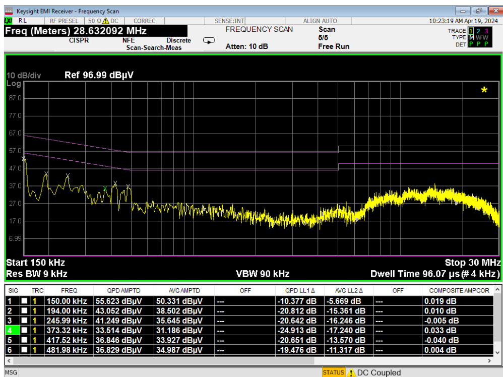
Plot 7-169. Line Conducted Plot with 802.11b (L1)_M1
