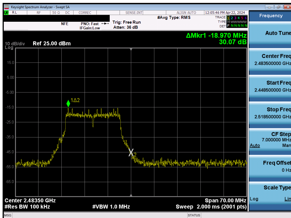
Plot 7-113. Band Edge Plot MIMO ANT2 (802.11g – Ch. 13)
