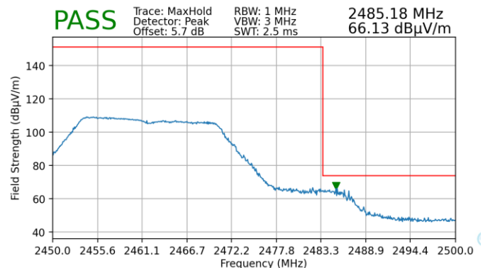
Plot 7-156. Radiated Restricted Upper Band Edge Measurement SISO ANT2 (Peak)
