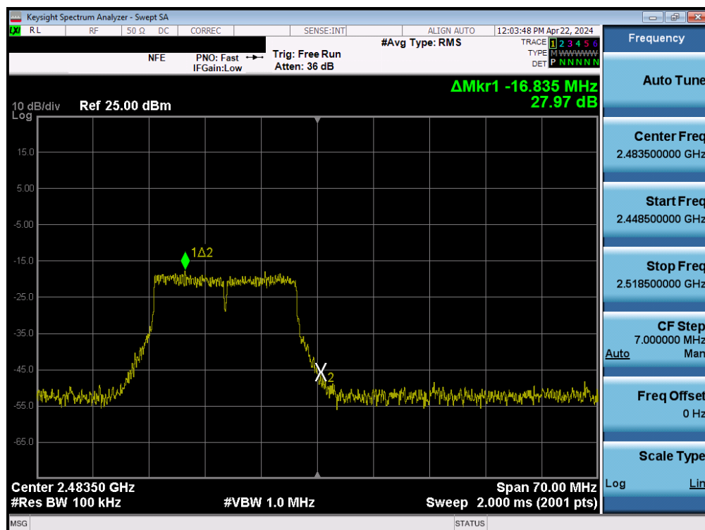
Plot 7-117. Band Edge Plot MIMO ANT2 (802.11n (2.4GHz) – Ch. 13)
