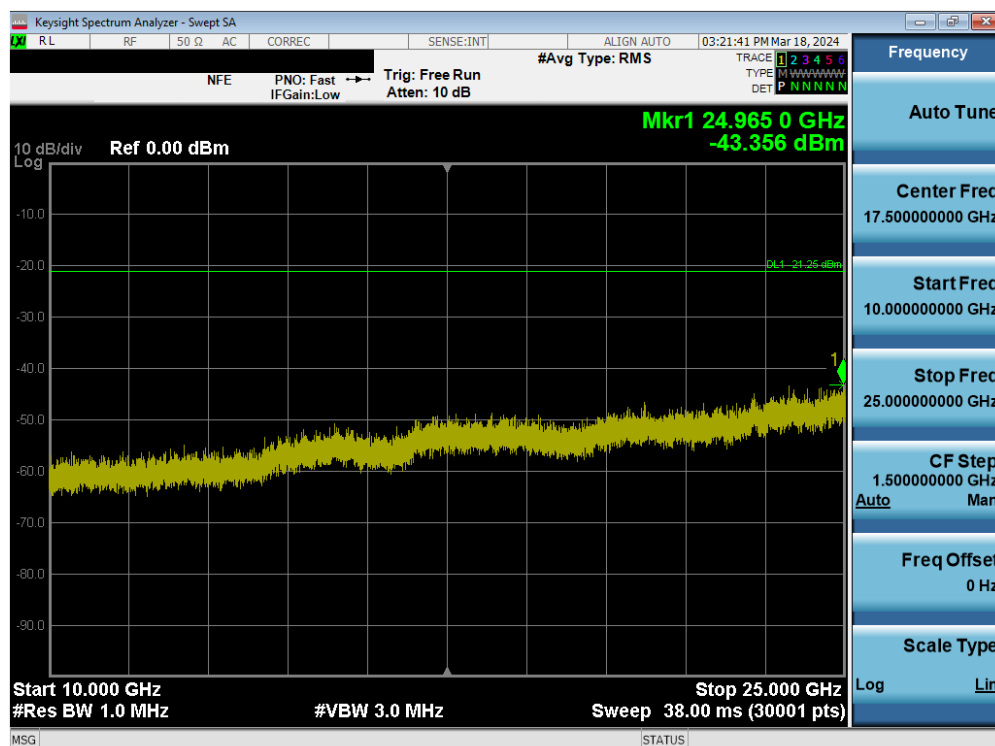
Plot 7-135. Conducted Spurious Plot MIMO ANT2 (802.11b – Ch. 1)
