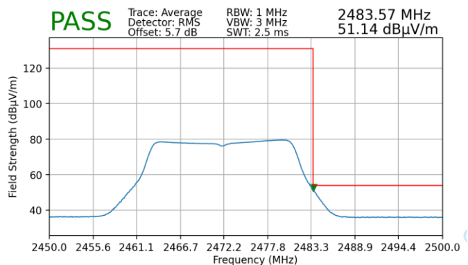
Plot 7-159. Radiated Restricted Upper Band Edge Measurement SISO ANT2 (Average)
