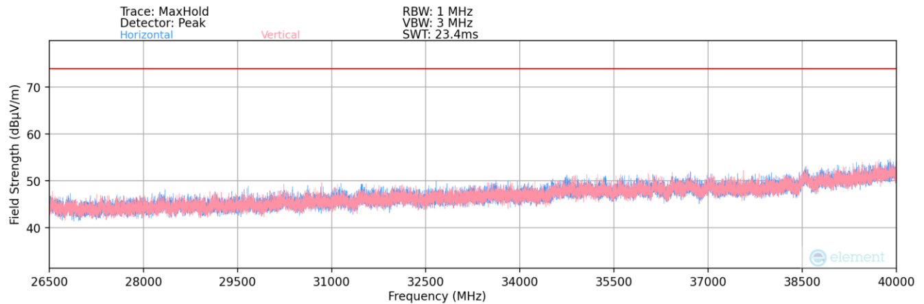
Plot 7-152. Radiated Spurious Plot above 26.5GHz (2.4GHz –6GHz)
