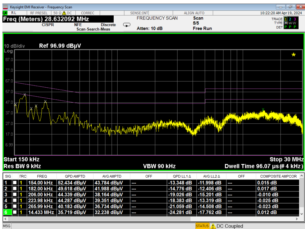
Plot 7-170. Line Conducted Plot with 802.11b (N)_M1
