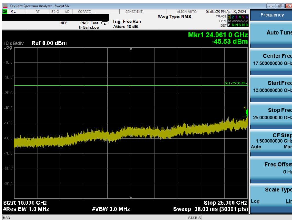
Plot 7-125. Conducted Spurious Plot SISO ANT2 (802.11b – Ch. 6)
