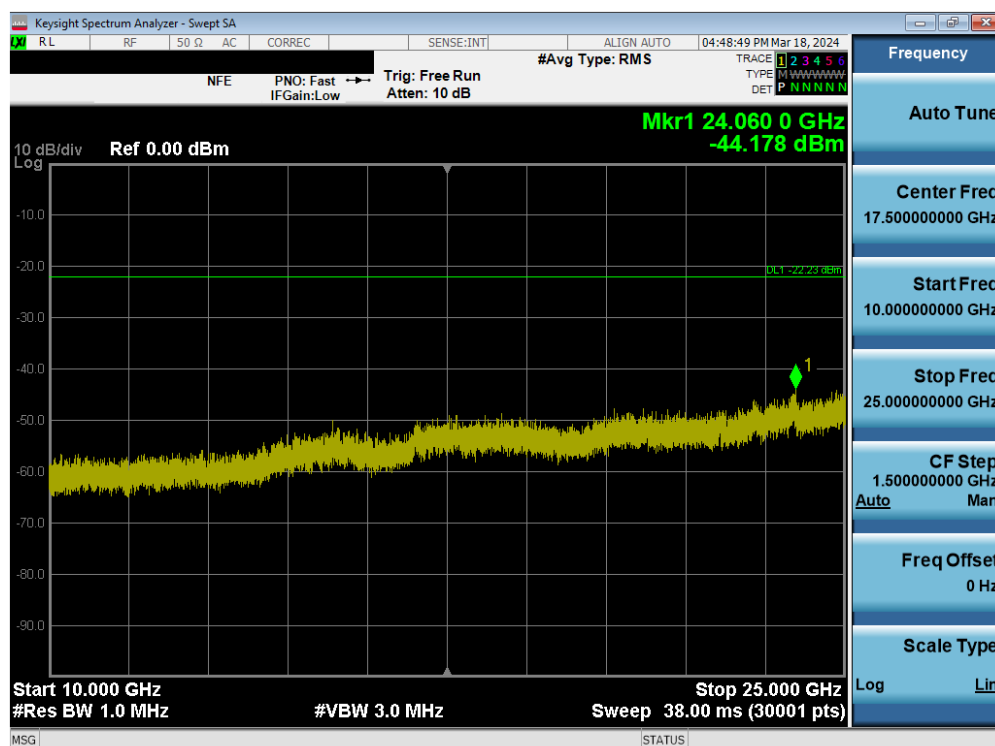
Plot 7-133. Conducted Spurious Plot MIMO ANT1 (802.11b – Ch. 11)
