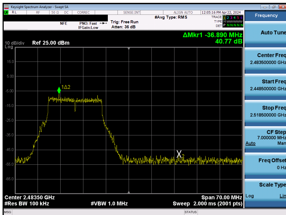
Plot 7-112. Band Edge Plot MIMO ANT2 (802.11g – Ch. 12)
