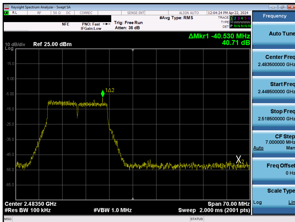
Plot 7-116. Band Edge Plot MIMO ANT2 (802.11n (2.4GHz) – Ch. 12)
