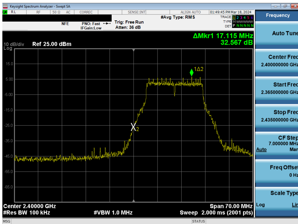
Plot 7-110. Band Edge Plot MIMO ANT2 (802.11g- Ch. 1)
