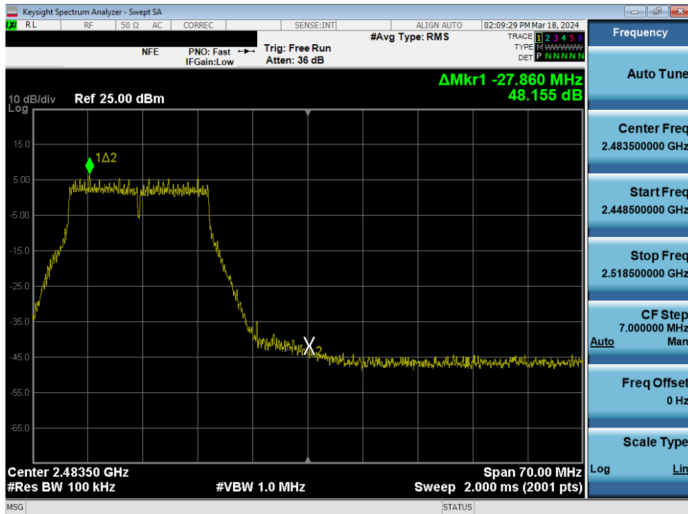
Plot 7-115. Band Edge Plot MIMO ANT2 (802.11n (2.4GHz) – Ch. 11)
