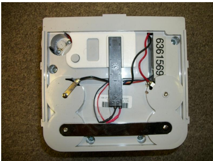
7.6 Georgia Pacific DIM Section Bottom View-with LF Antenna
