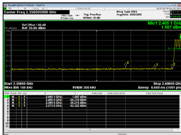
Band-edge Emission
