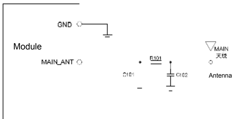
Figure 39 MAIN Antenna Interface Simplified Connection Circuit
