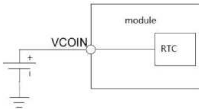
Figure 19 Rechargeable Battery Powers RTC
