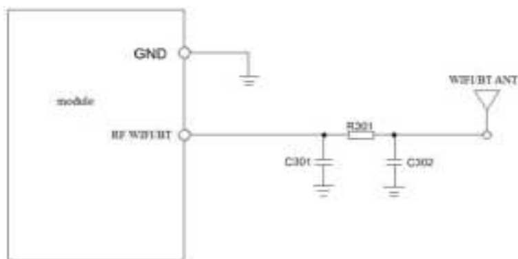
Figure 44 WIFI_BT antenna interface simplified connection circuit
