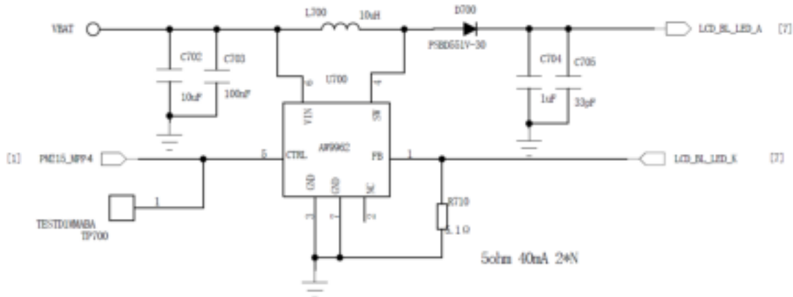
Figure 24 Backlight drive schematic
