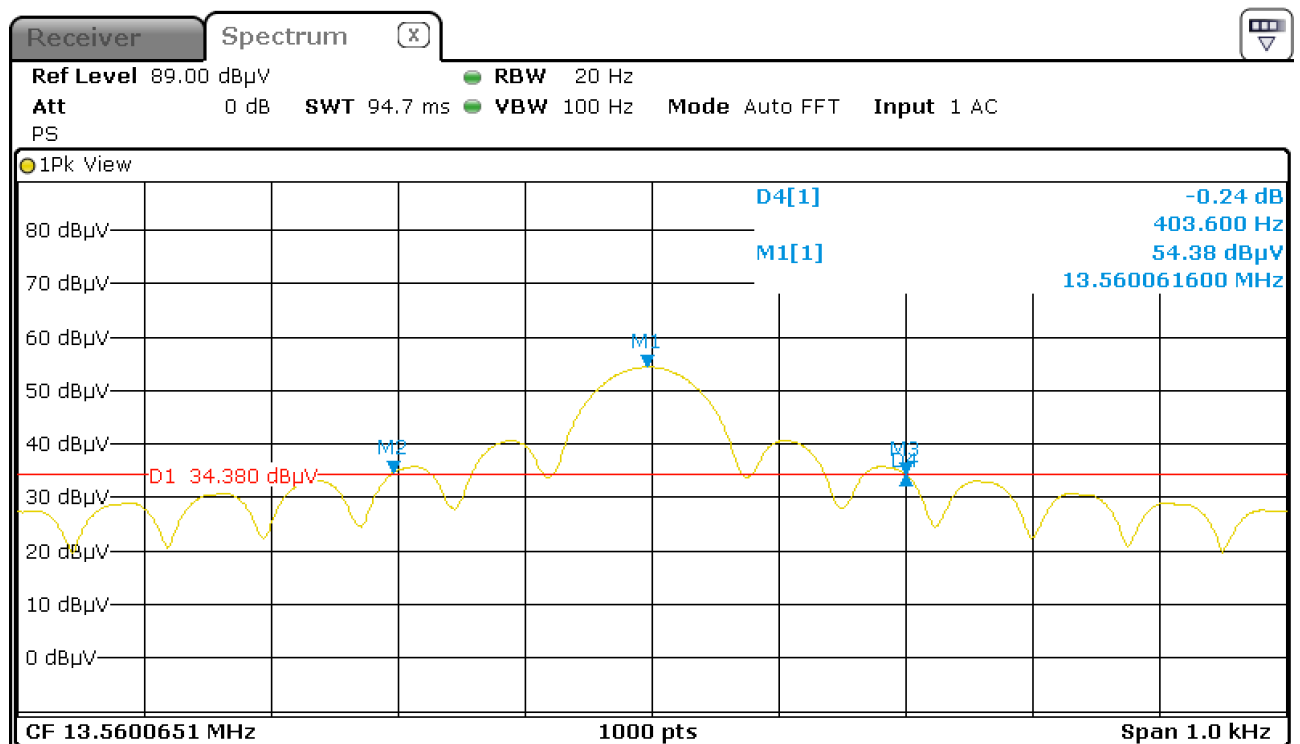
Figure 8: Chart of 20 dB bandwidth tests at normal conditions, without tag
