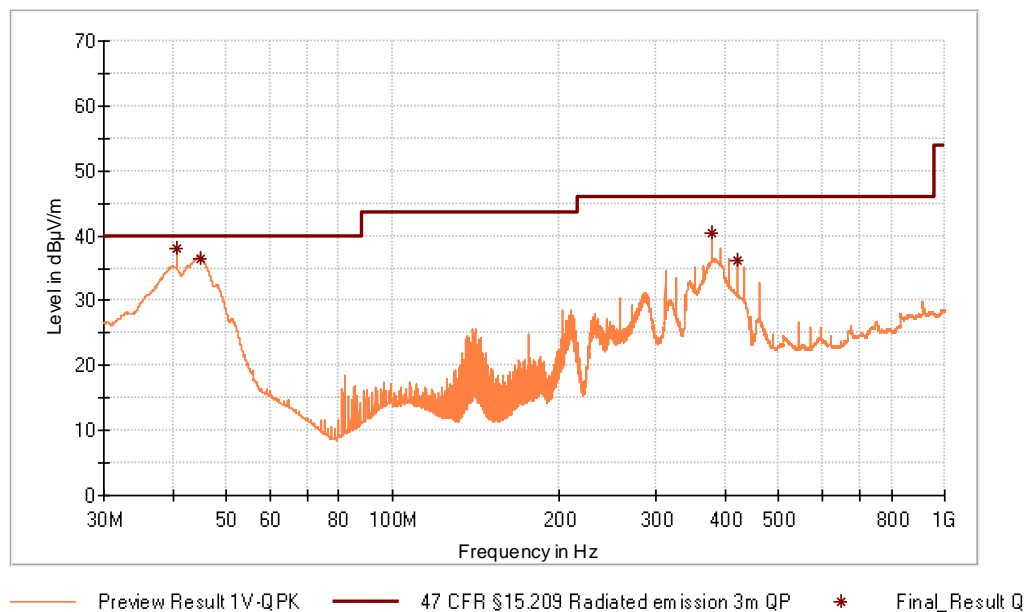
Figure 12: Chart of radiated emissions test from 30 MHz to 1 GHz, EUT position Y, antenna polarization vertical, with tag
