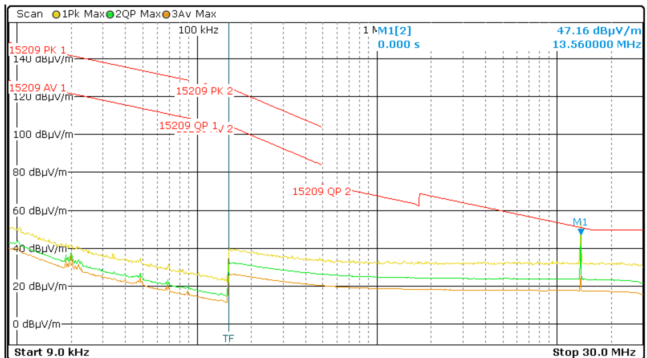
Figure 11: Chart of radiated emissions test below 30 MHz, EUT position Y, antenna polarization in line, without tag
