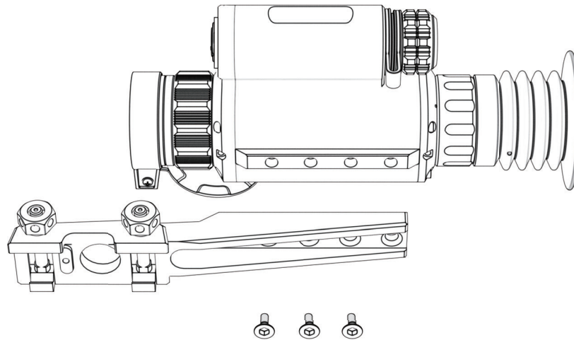
Figure 23 Mount Installation
