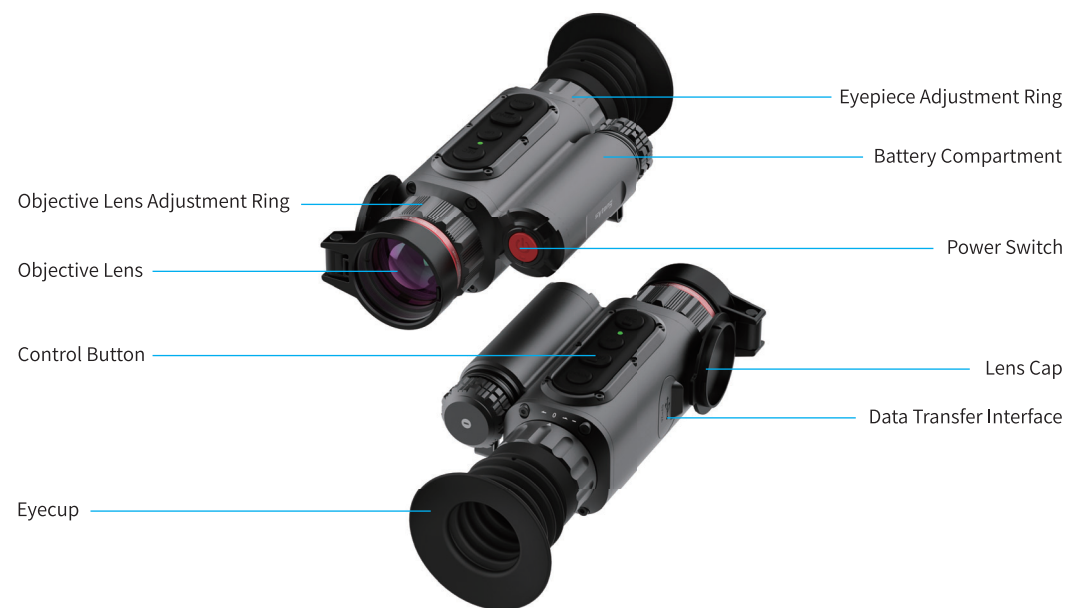
Figure 2 Thermal Imaging Scope Component
