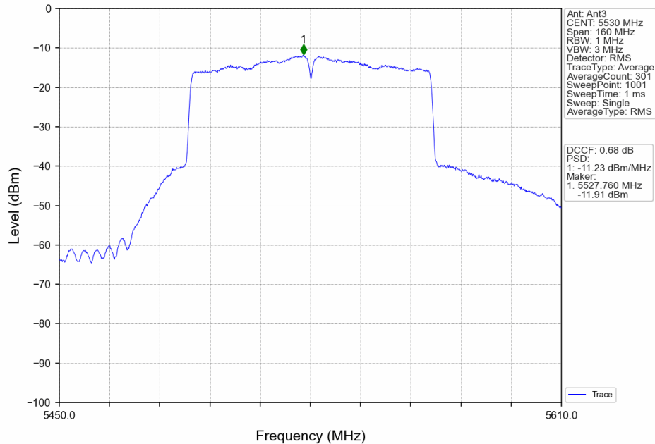
802.11ac(VHT80)_LCH_5530MHz_MIMO_NTNV
