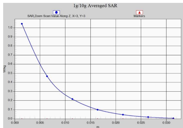
Fig. 1-38 Z-Scan at power reference point (LTE Band7)
