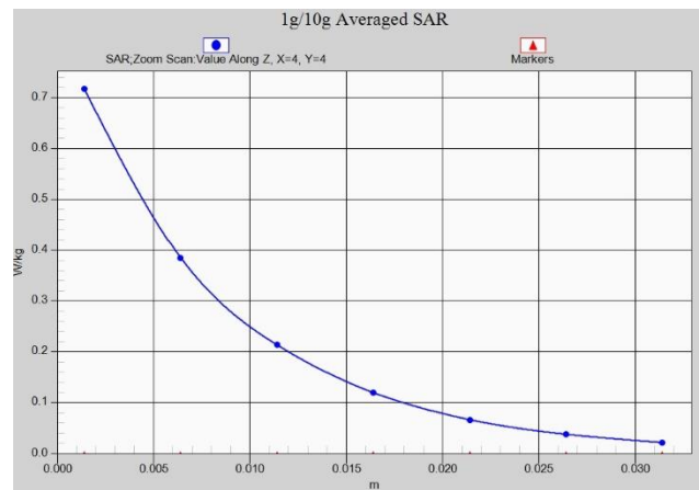
Fig. 1-43 Z-Scan at power reference point (LTE Band66)
