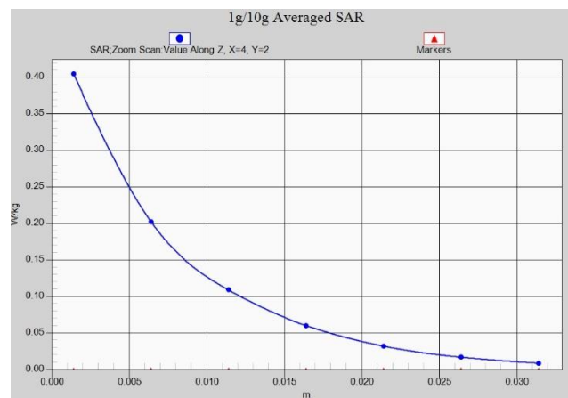
Fig. 1-44 Z-Scan at power reference point (LTE Band66)
