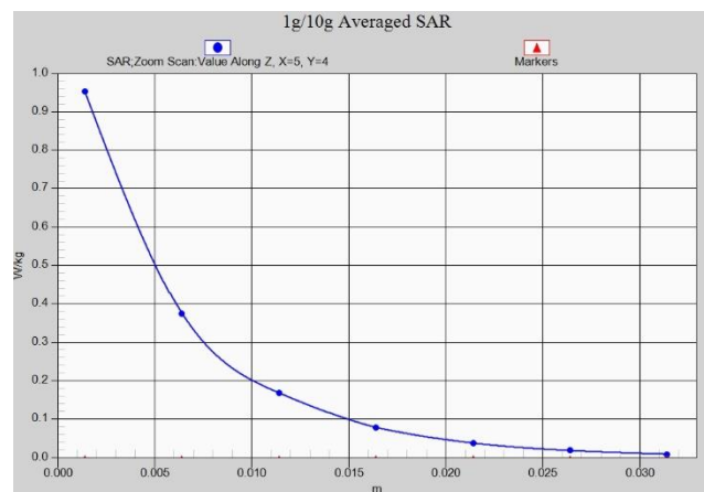
Fig. 1-45 Z-Scan at power reference point (wifi2450)
