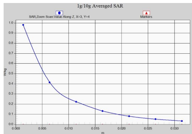
Fig. 1-35 Z-Scan at power reference point (LTE Band5)
