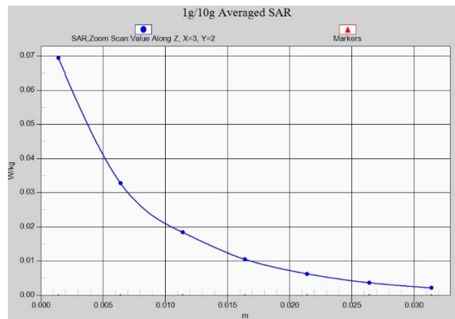
Fig. 1-40 Z-Scan at power reference point (LTE Band12)
