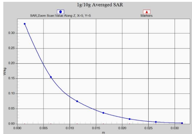
Fig. 1-46 Z-Scan at power reference point (wifi2450)
