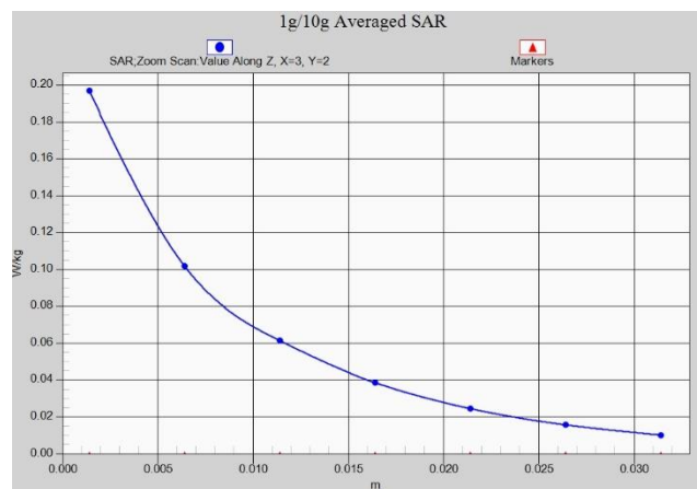
Fig. 1-32 Z-Scan at power reference point (WCDMA850)
