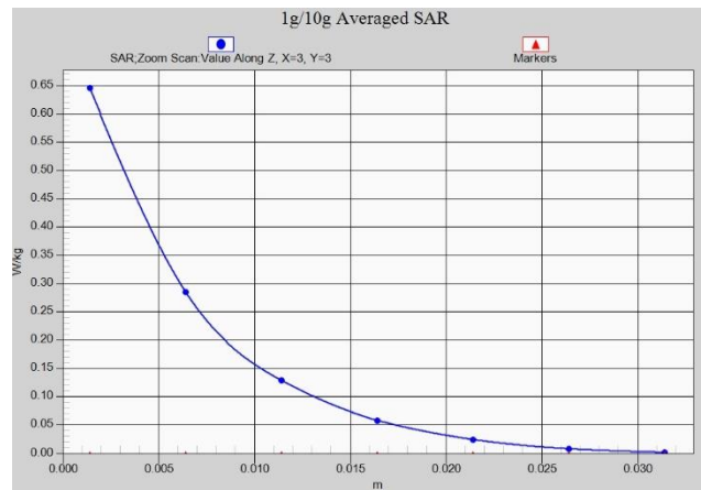
Fig. 1-42 Z-Scan at power reference point (LTE Band41)
