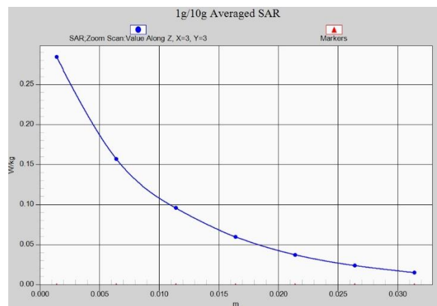
Fig. 1-36 Z-Scan at power reference point (LTE Band5)
