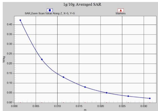
Fig. 1-31 Z-Scan at power reference point (WCDMA850)
