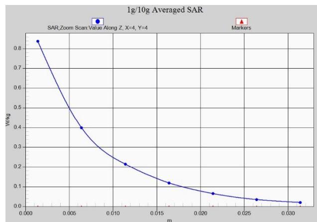
Fig. 1-33 Z-Scan at power reference point (LTE Band2)
