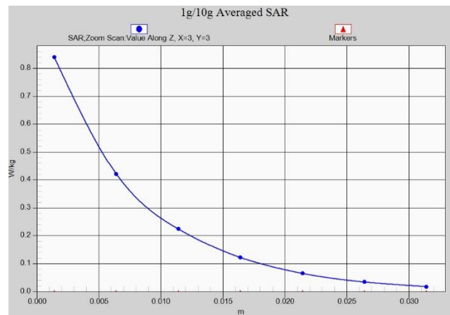
Fig. 1-34 Z-Scan at power reference point (LTE Band2)
