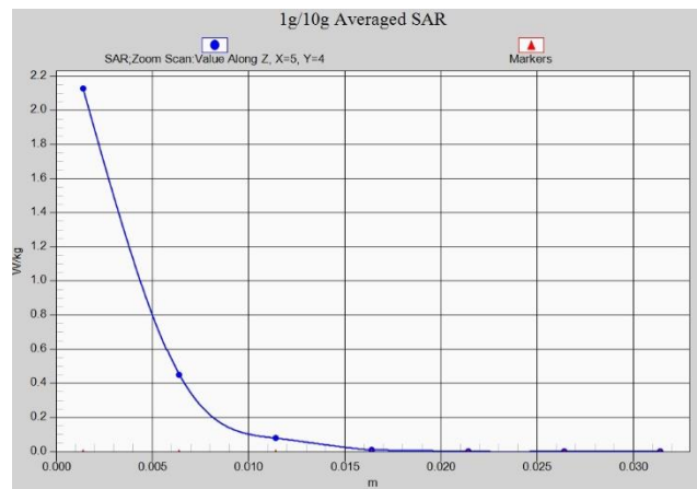
Fig. 1-47 Z-Scan at power reference point (wifi5G)
