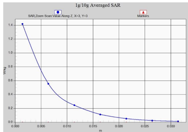
Fig. 1-37 Z-Scan at power reference point (LTE Band7)
