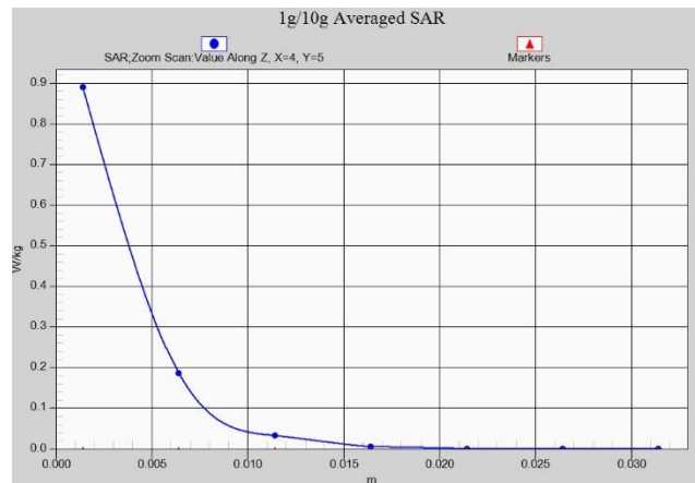
Fig. 1-48 Z-Scan at power reference point (wifi5G)
