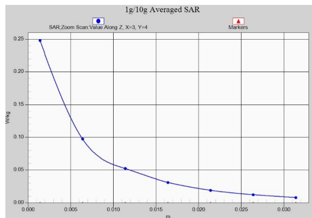
Fig. 1-39 Z-Scan at power reference point (LTE Band12)
