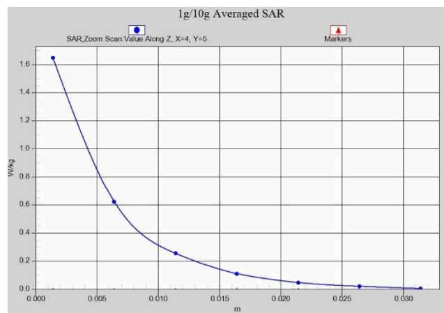
Fig. 1-41 Z-Scan at power reference point (LTE Band41)
