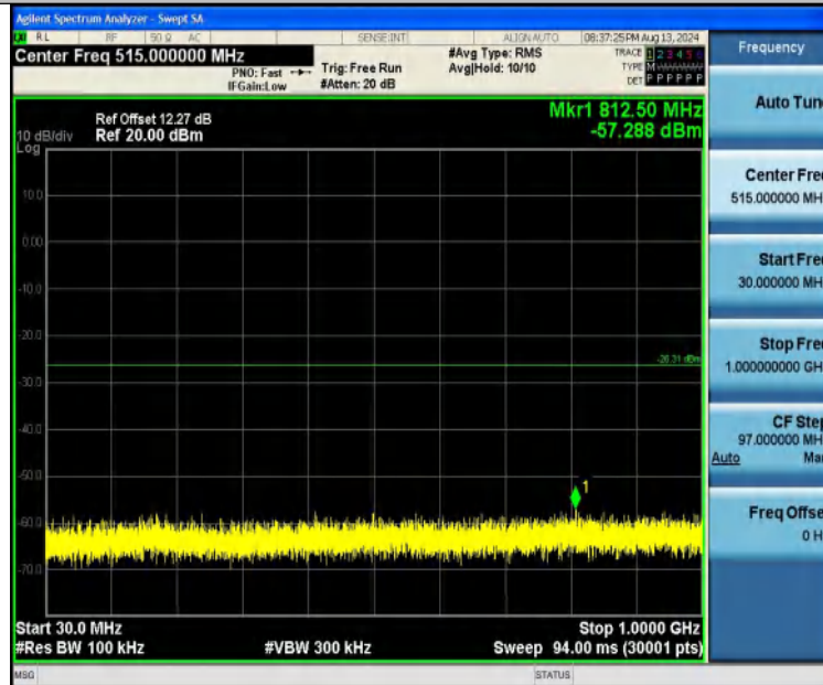
11N40SISO-Ant1-2437-30~1000-PASS
