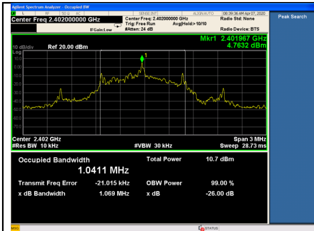
BLE-OBW-Low
