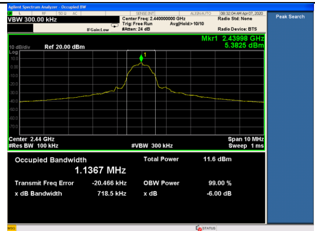
BLE-DTS BW-Mid
