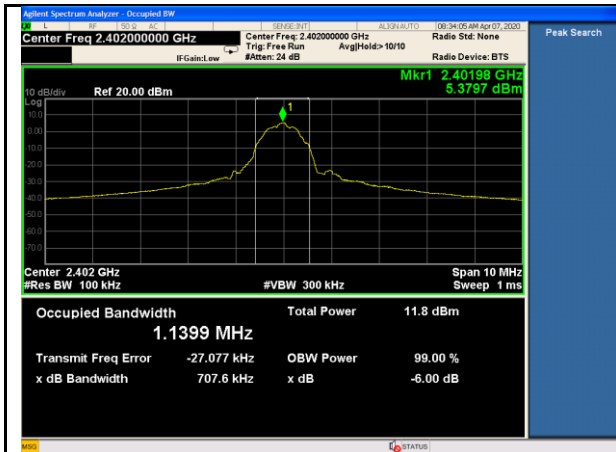
BLE-DTS BW-Low
