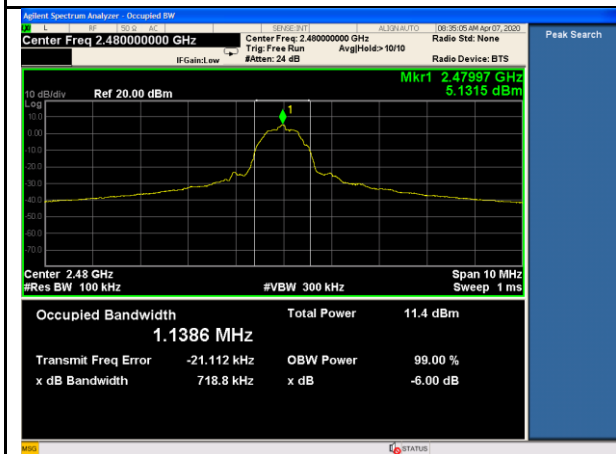
BLE-DTS BW-High
