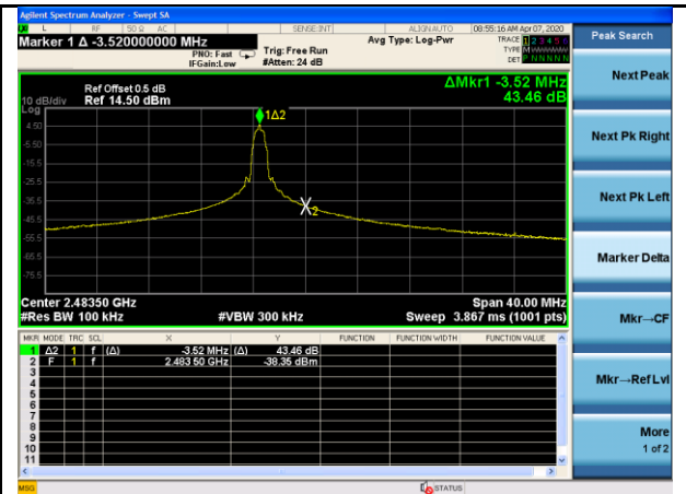
BLE-Band Edge-High
