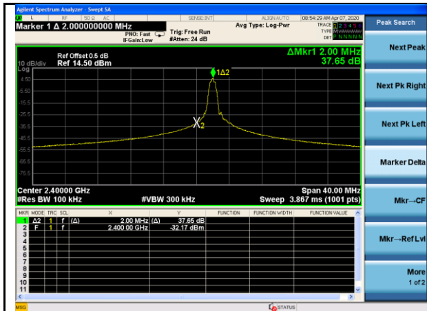
BLE-Band Edge-Low
