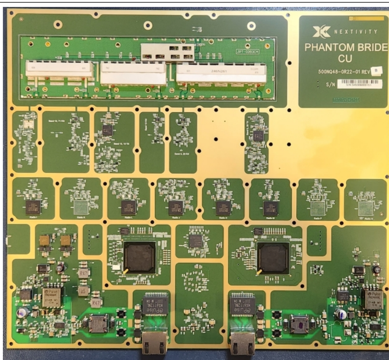
PCB side 2
