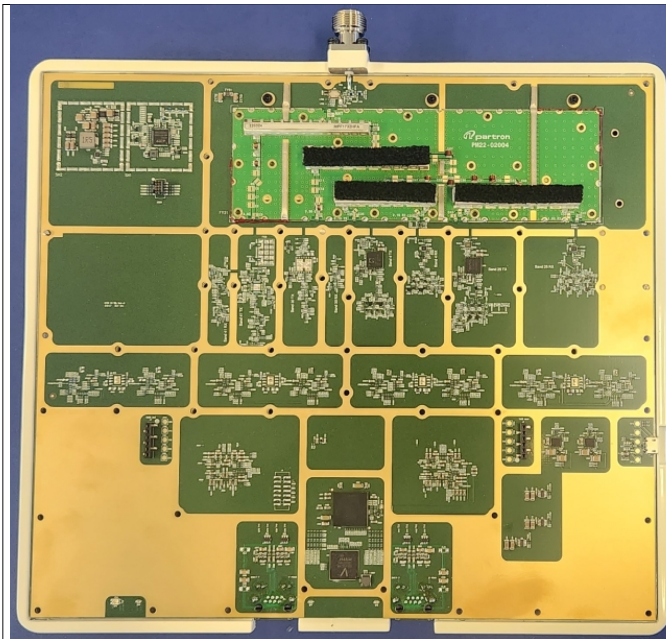
PCB Side 1
