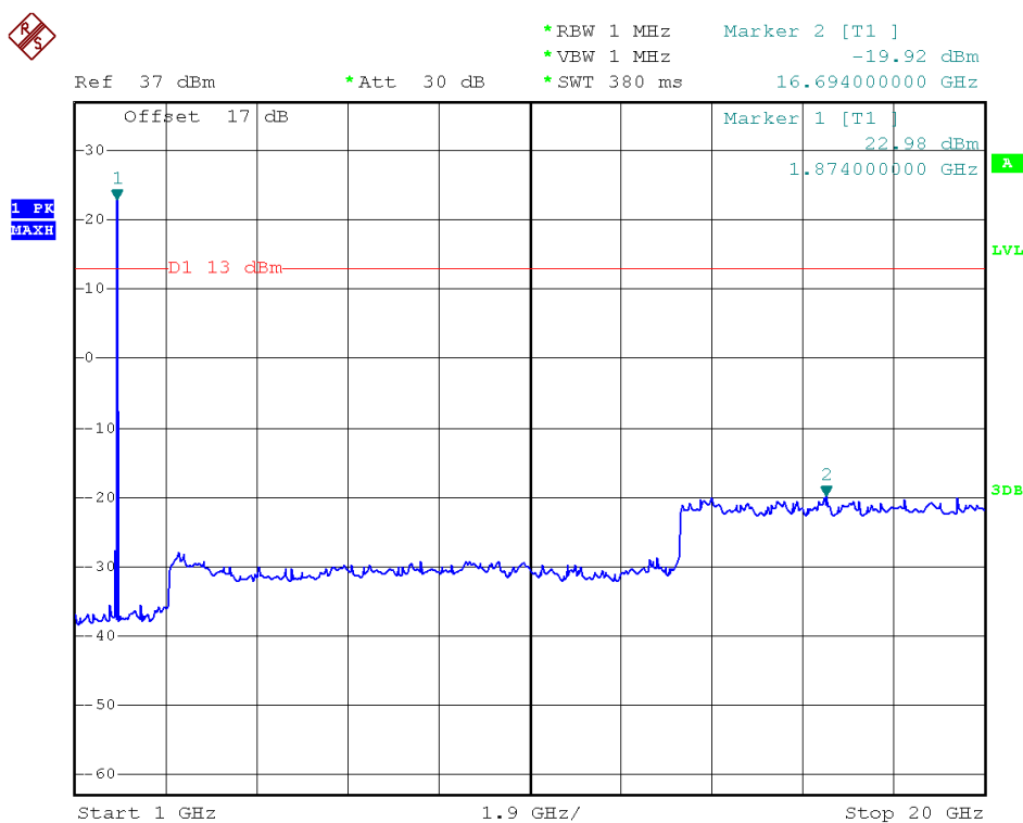
WCDMA1900MHz Channel = 9400, 1GHz to 20GHz
