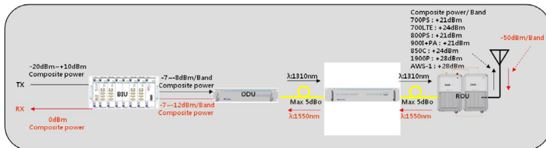
Figure 6.16 –SC-DAS Link Budget for OEU
