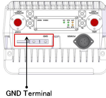
Figure 5.24 – ROU GND Port view
