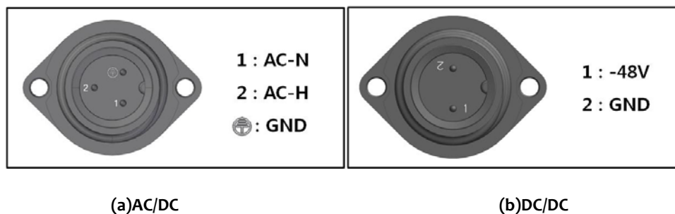
Figure 5.22 – ROU Power Port view
