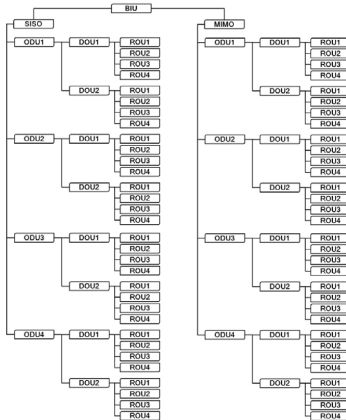
Figure 6.7 –Configuration of BIU-ODU-ROU for basic topology
