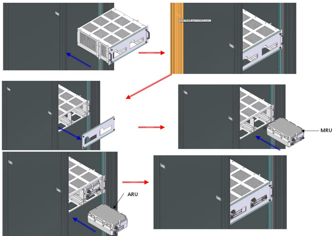
Figure 5.20 – ROU installation procedure for horizontal rack
