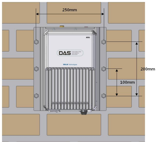
Figure 5.17 – ROU installation diagram for stacked mounting
