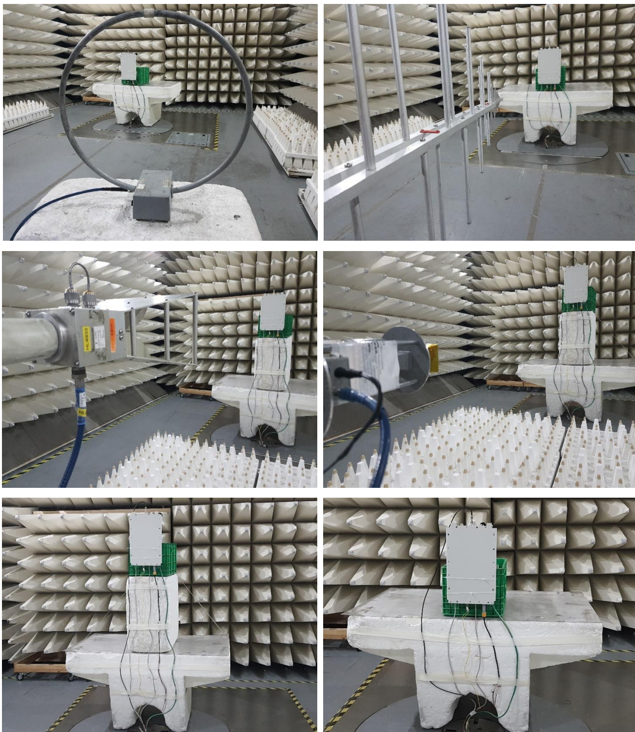
Photograph 7.4.1 Setup for radiated emission measurements
