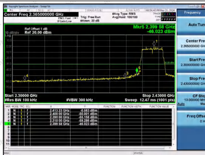
11G-Ant1-2412-PASS
