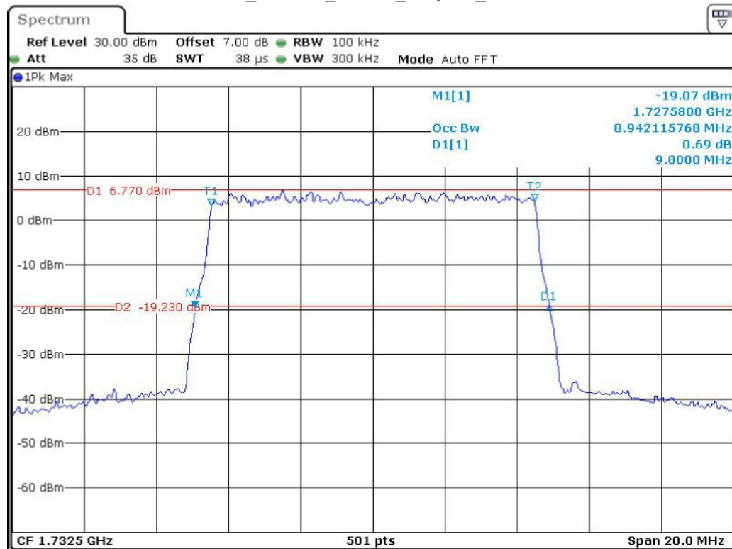
Band 4_10 MHz_Middle_16QAM_RB50#0
