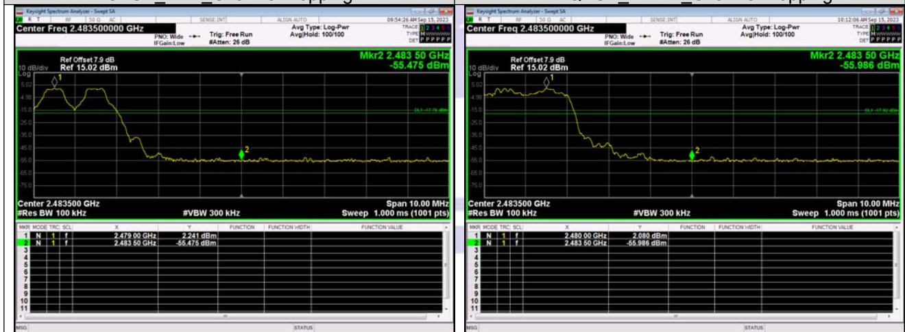
Out Of Band Emission(Right)
