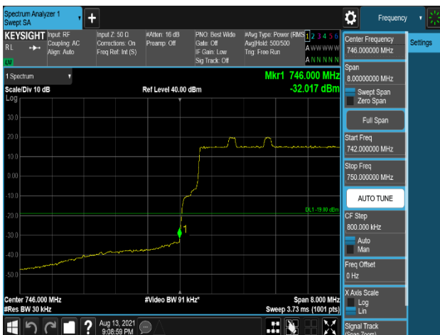
Plot 7-319. Band Edge Emission (745.9MHz to 746MHz) Plot (LTE_B13_10M+Low_NB-IoT(IB)+Low_NB-IoT(IB)_1C - Port 3)
