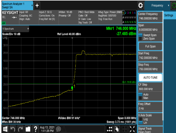
Plot 7-315. Band Edge Emission (745.9MHz to 746MHz) Plot (LTE_B13_5M+NB-IoT(IB)_1C - Port 3)
