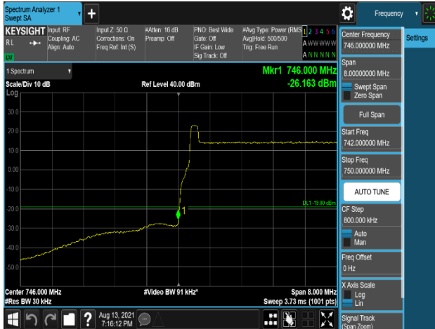
Plot 7-323. Band Edge Emission (745.9MHz to 746MHz) Plot (LTE_B13_10M+Low_NB-lot(GB)+High_NB-lot(GB)_3C – Port 0)
