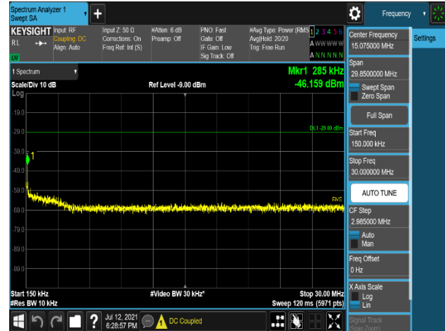
Plot 7-342. Conducted Spurious Emission Plot 150 kHz to 30 MHz (LTE_B5_5M_1C_256QAM - Low Channel, Port 2)
