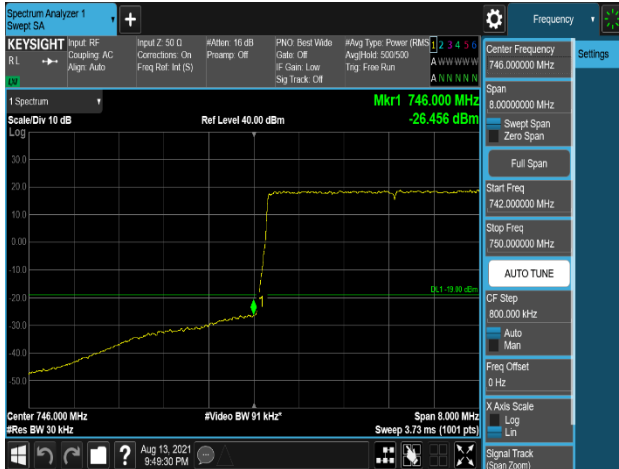
Plot 7-309. Band Edge Emission (745.9MHz to 746MHz) Plot (LTE_B13_5M_1C_64QAM - Low Channel, Port 1)
