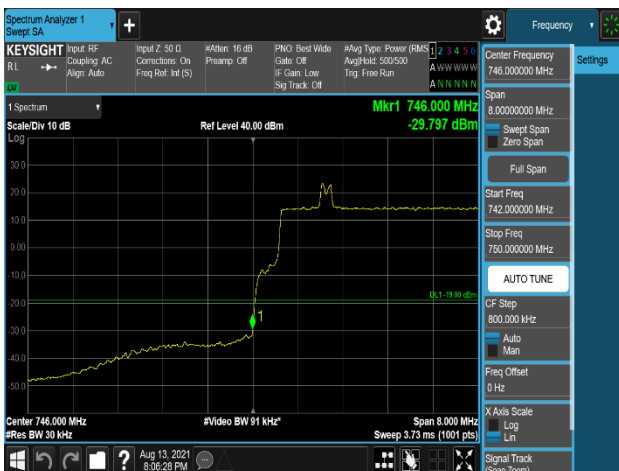
Plot 7-327. Band Edge Emission (745.9MHz to 746MHz) Plot (LTE_B13_10M+High_NB-lot(GB)+Low_NB-lot(IB)_2C – Port 0)
