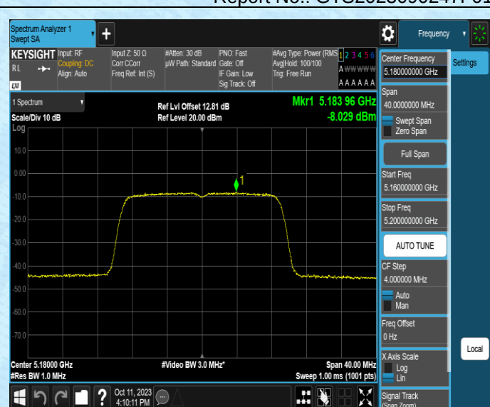
11AC20SISO-Ant2-5180-PASS
