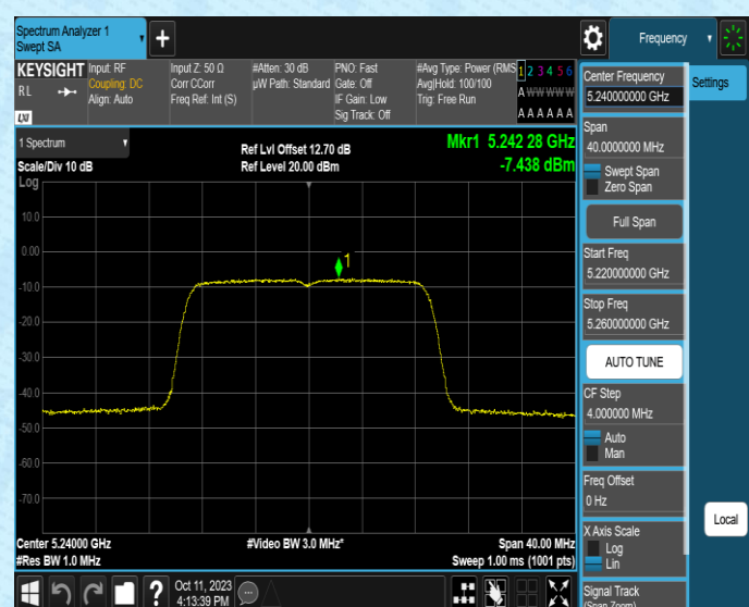
11AC20SISO-Ant2-5240-PASS
