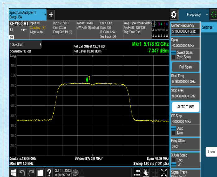
11AC20SISO-Ant1-5180-PASS
