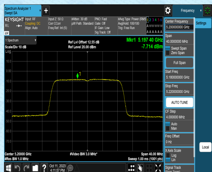
11AC20SISO-Ant2-5200-PASS
