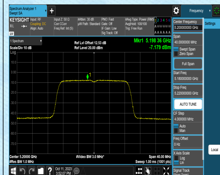
11AC20SISO-Ant1-5200-PASS
