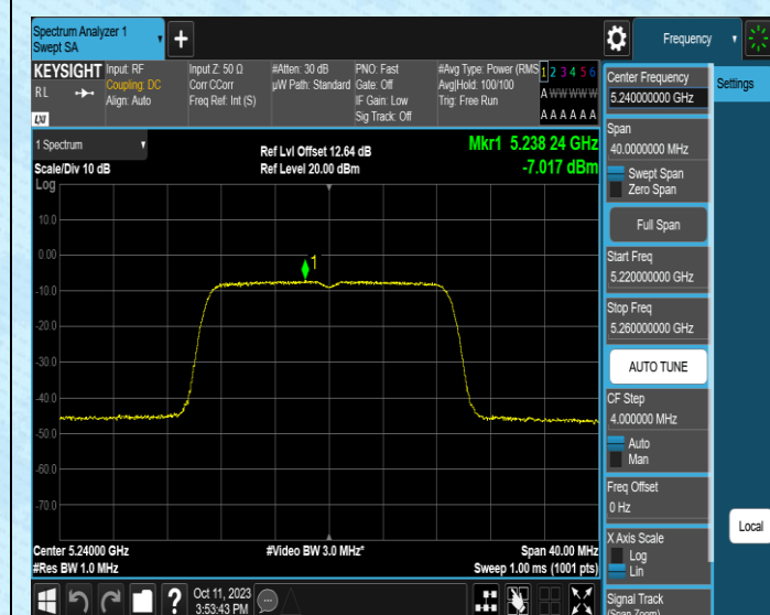
11AC20SISO-Ant1-5240-PASS
