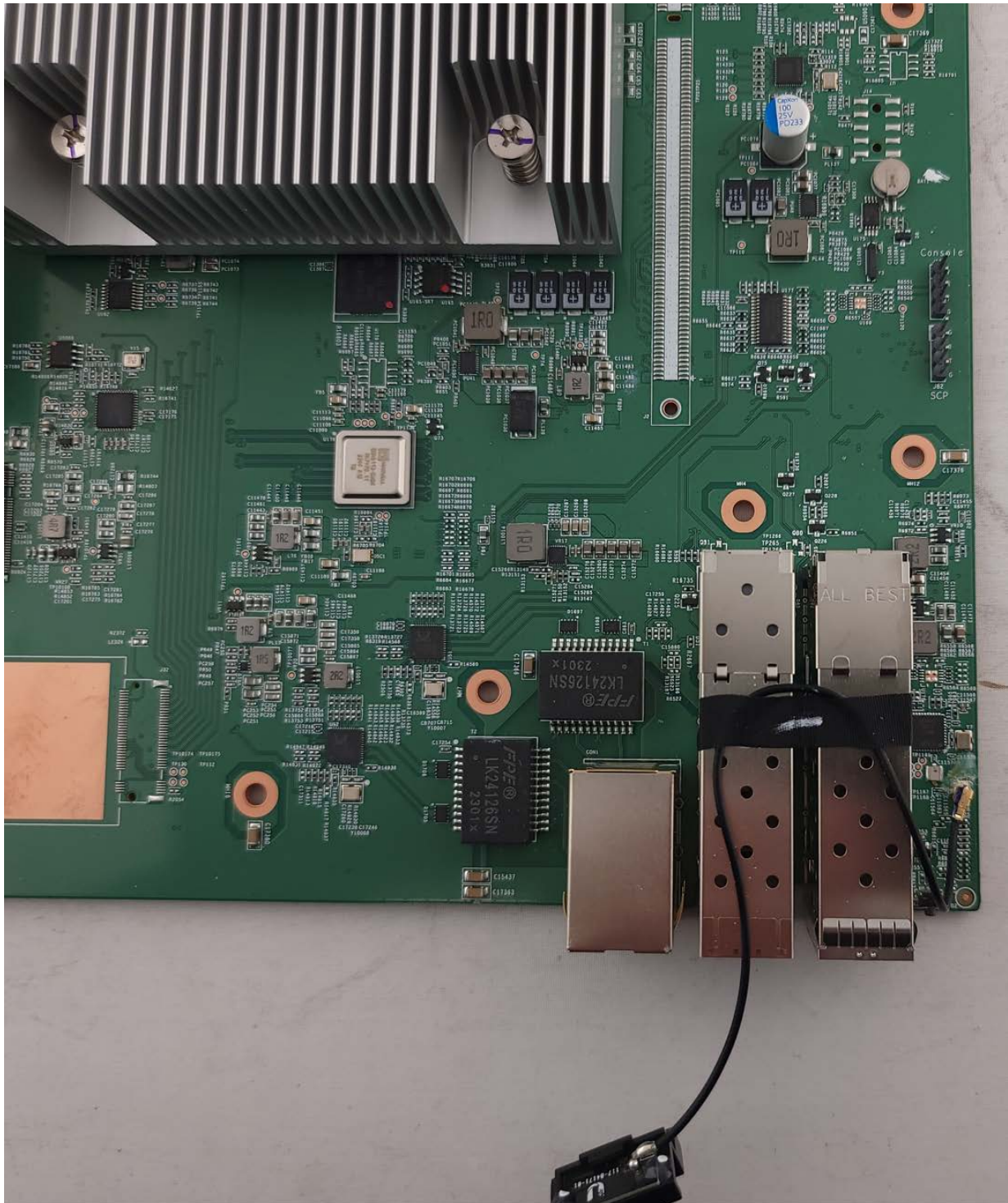
Photograph 1: Top Main PCB Close-up Front/Right
