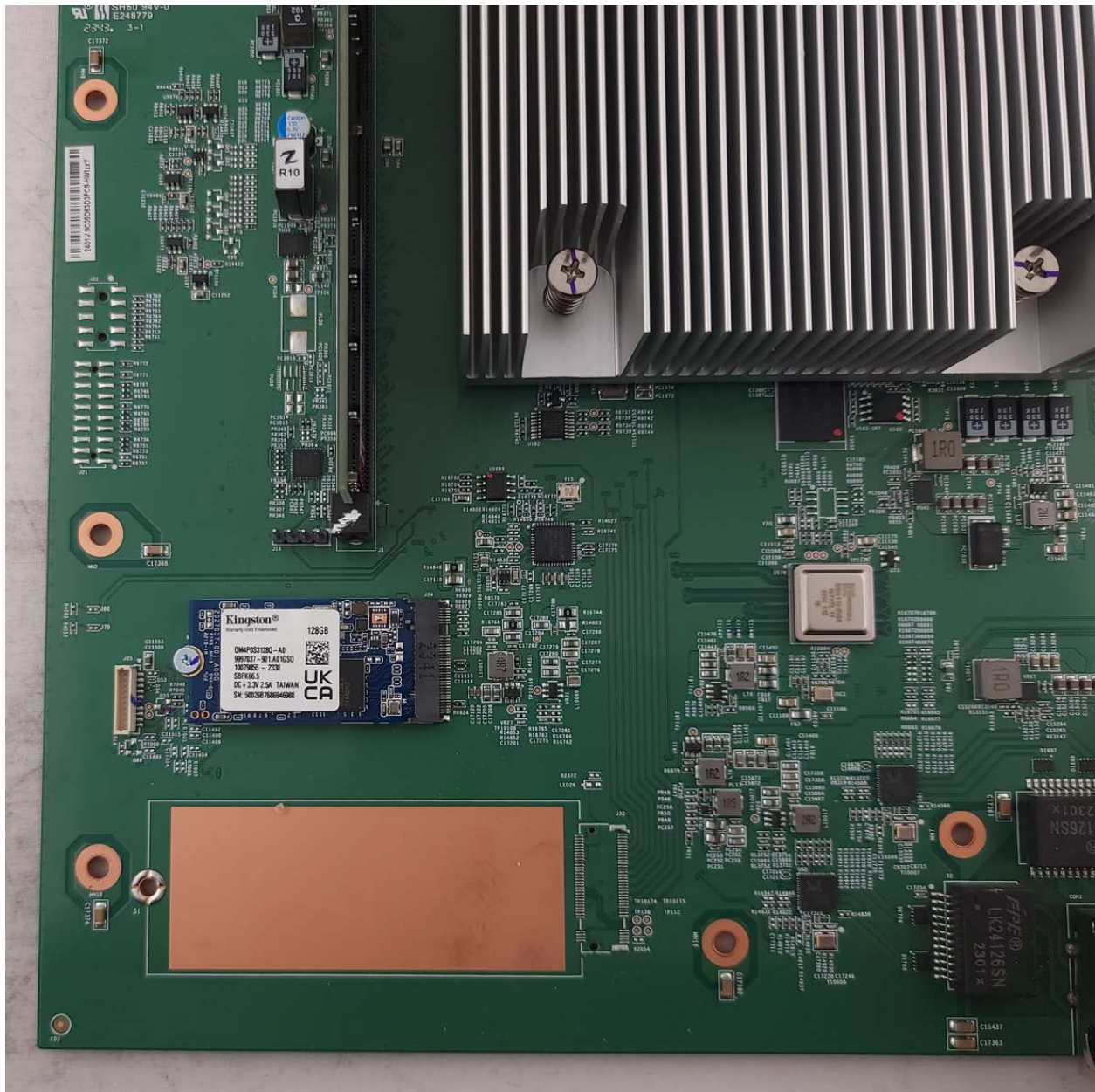
Photograph 2: Top Main PCB Close-up Front/Left
